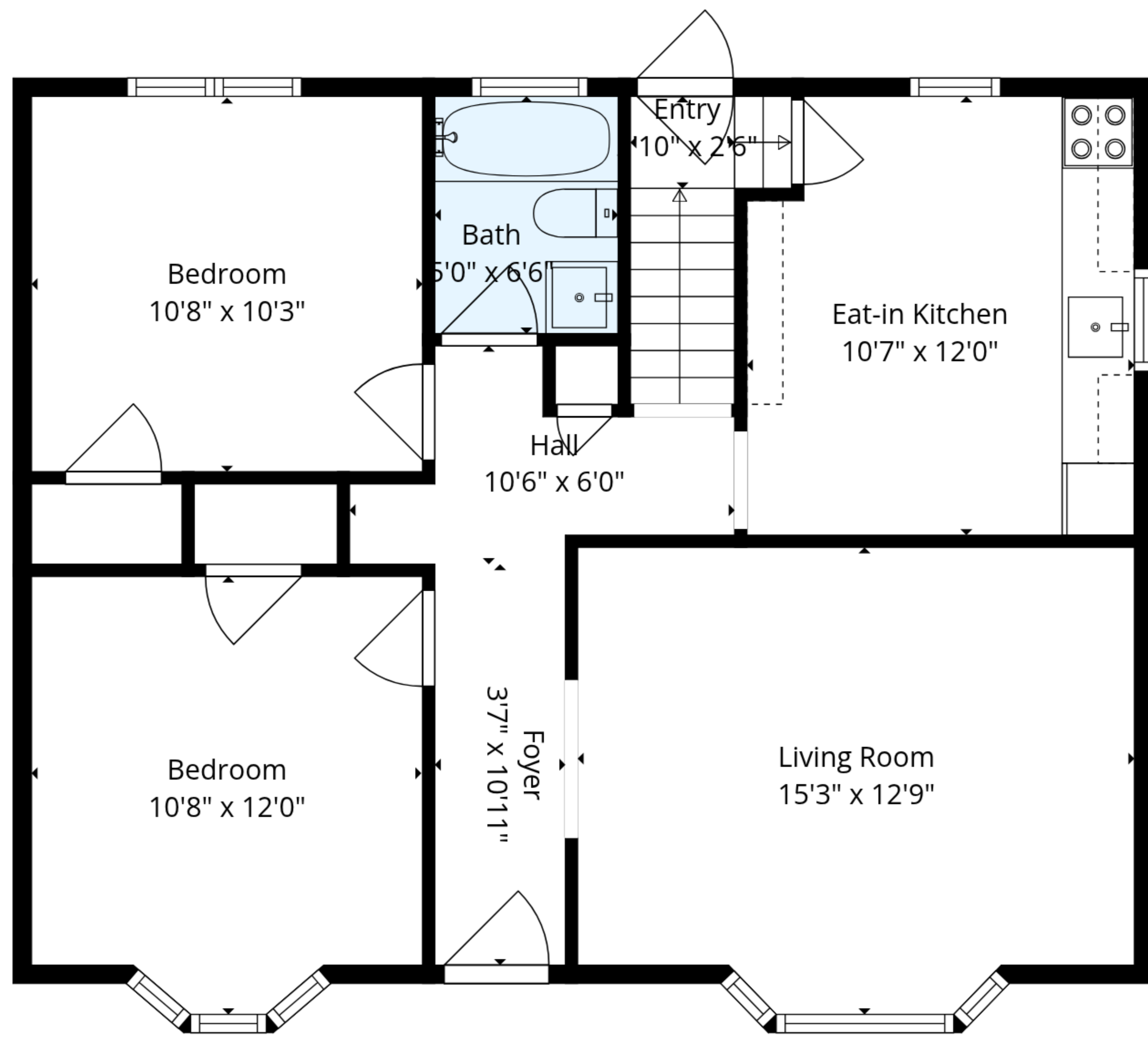
1st Floor
