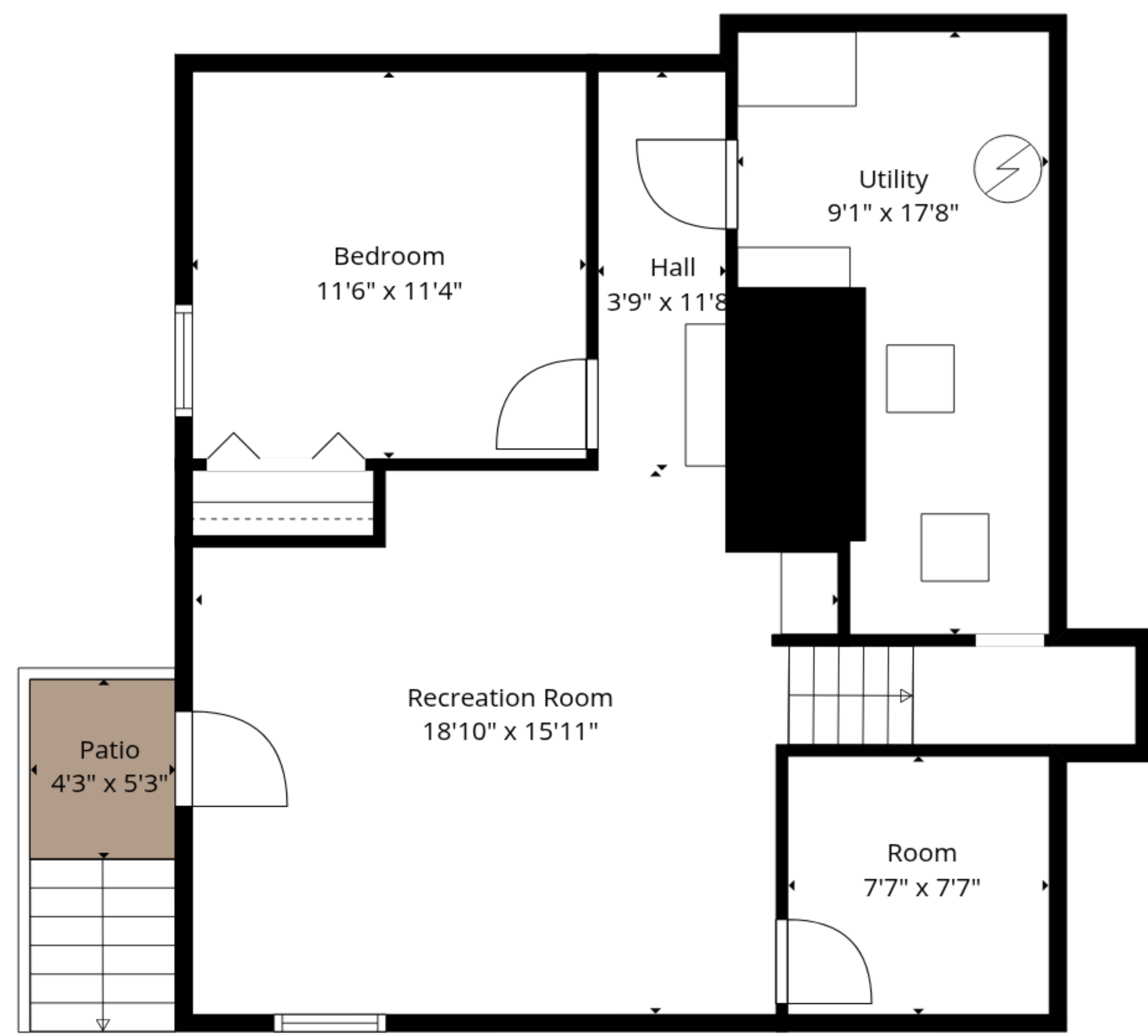
Basement
