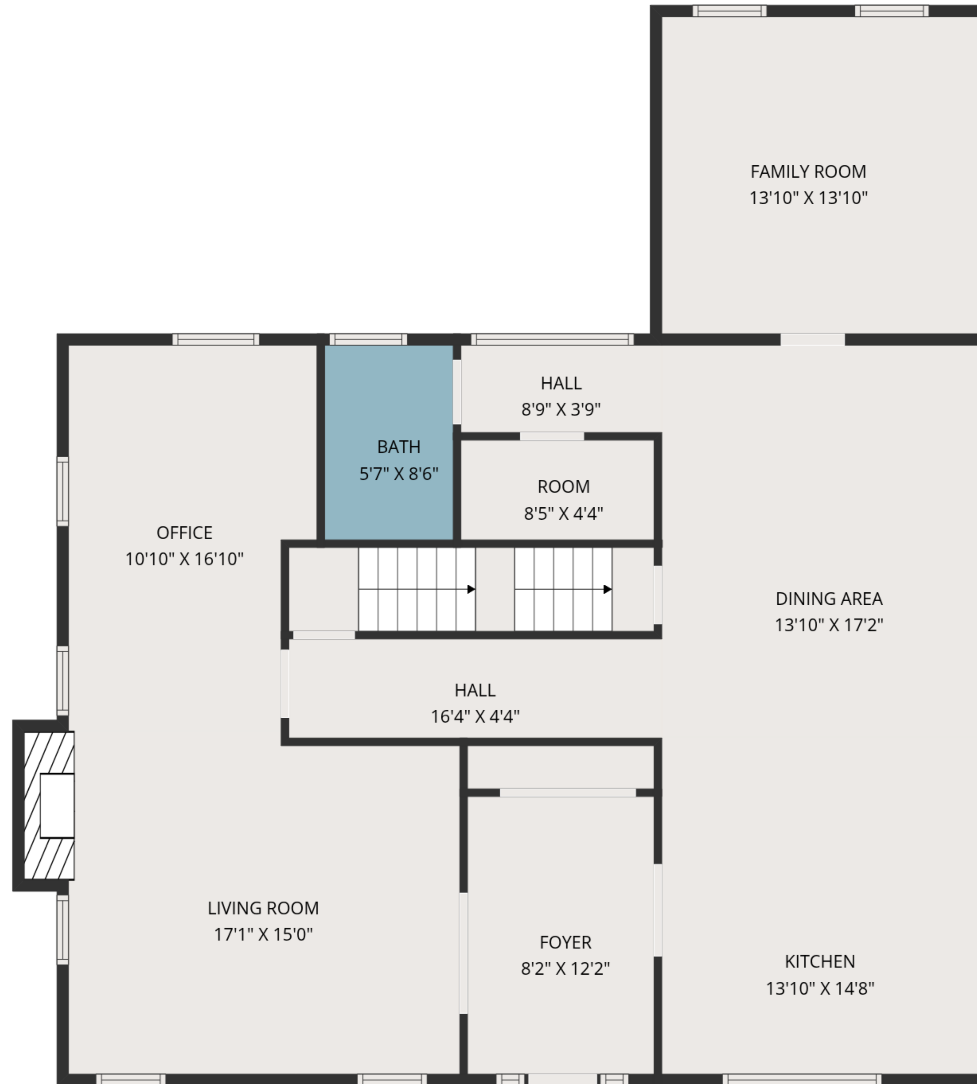
2ND FLOOR
