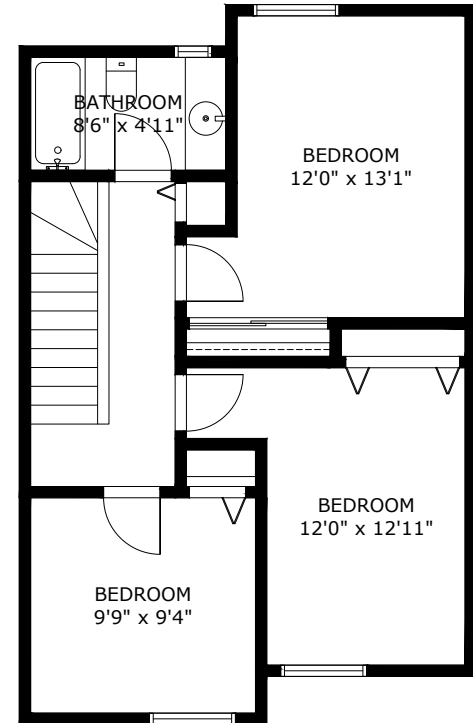
Upper Level Area: Ceiling Height: 8'0"
