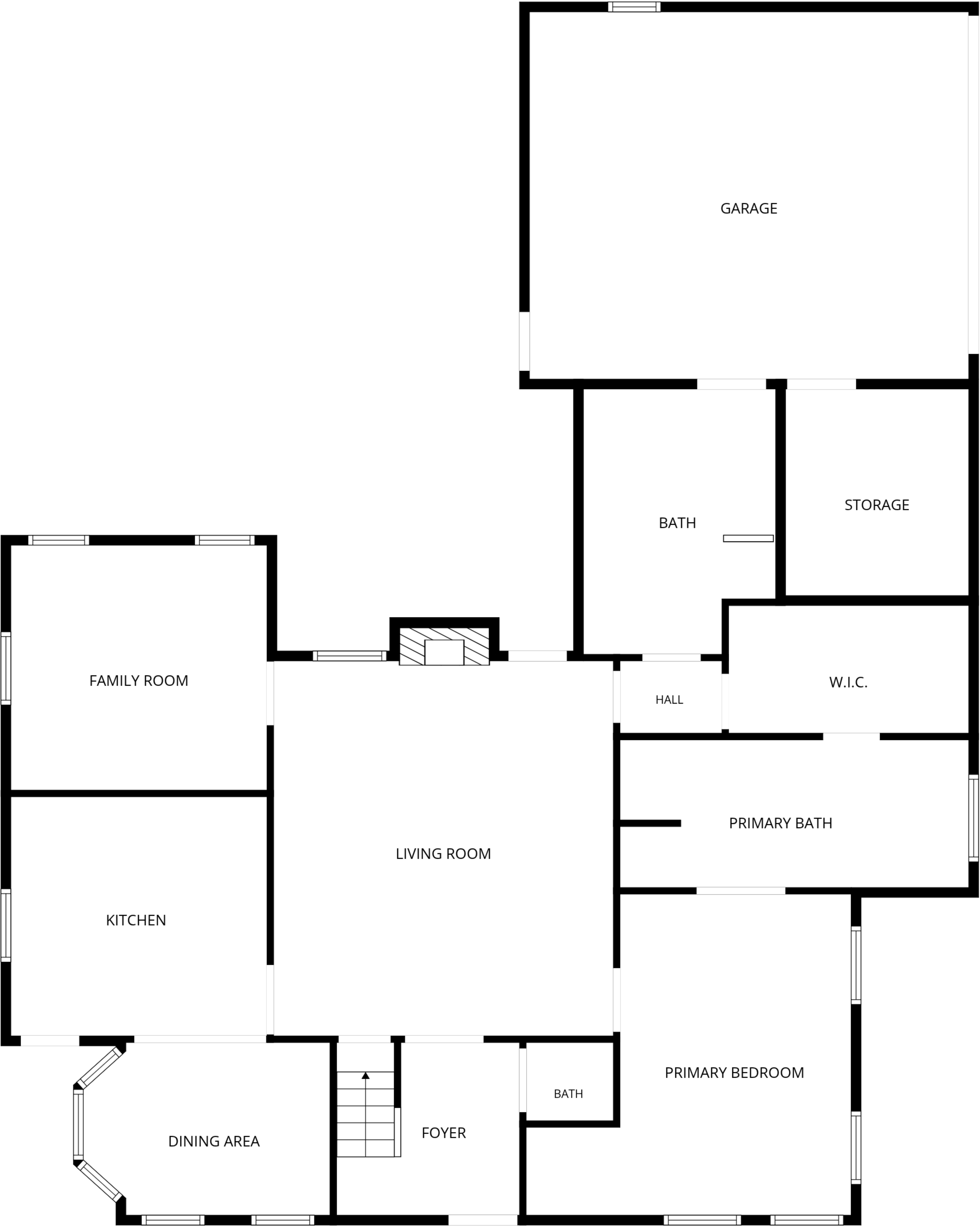
1st floor
