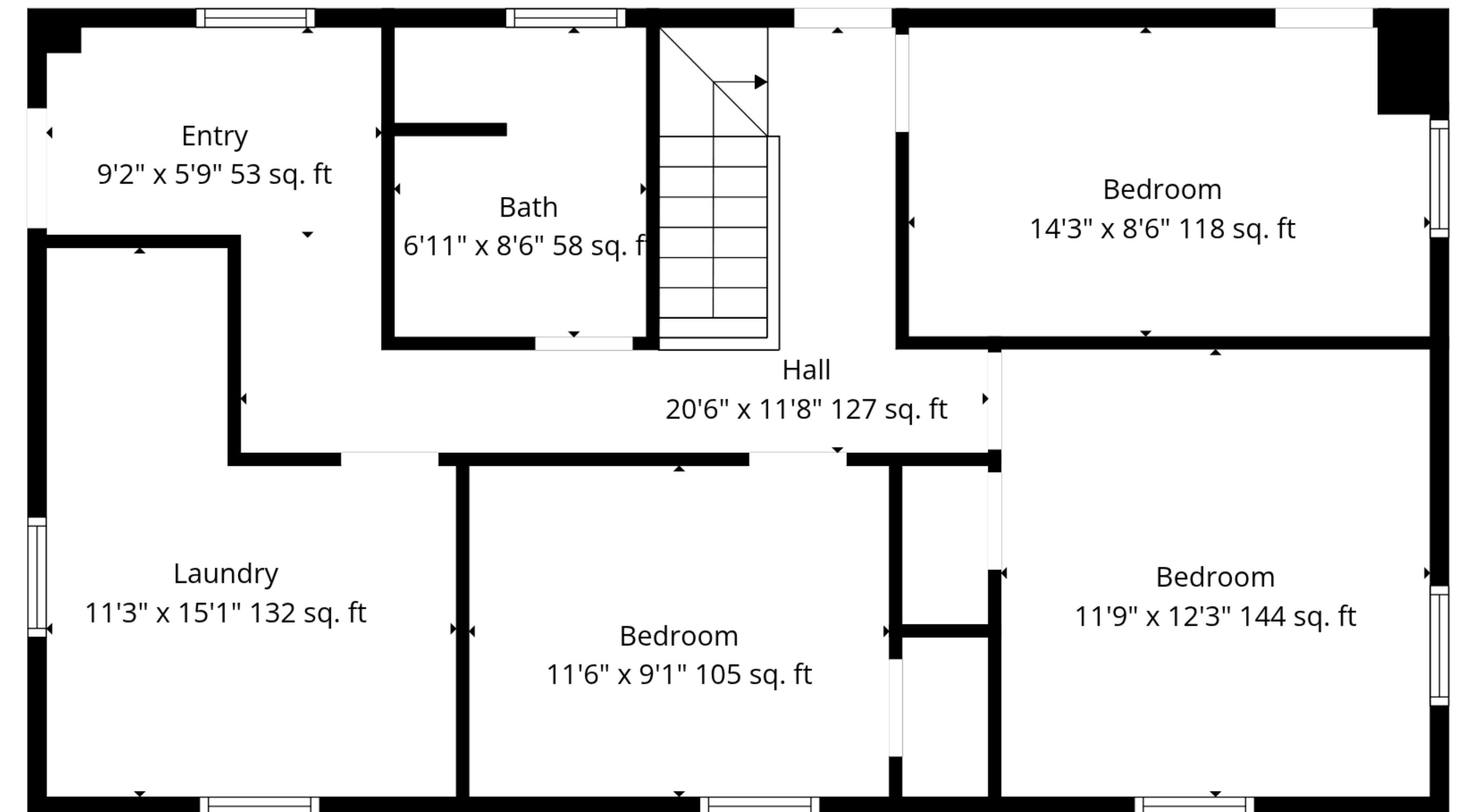
2nd Floor
