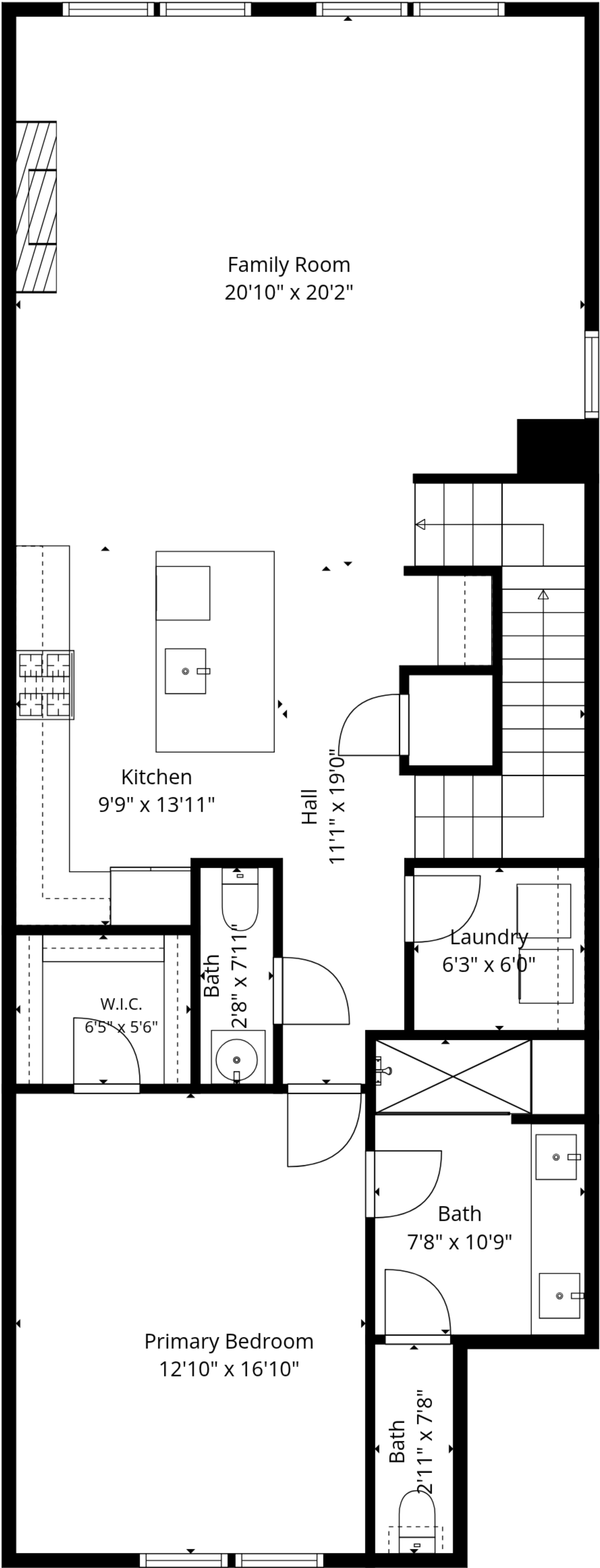
2nd Floor
