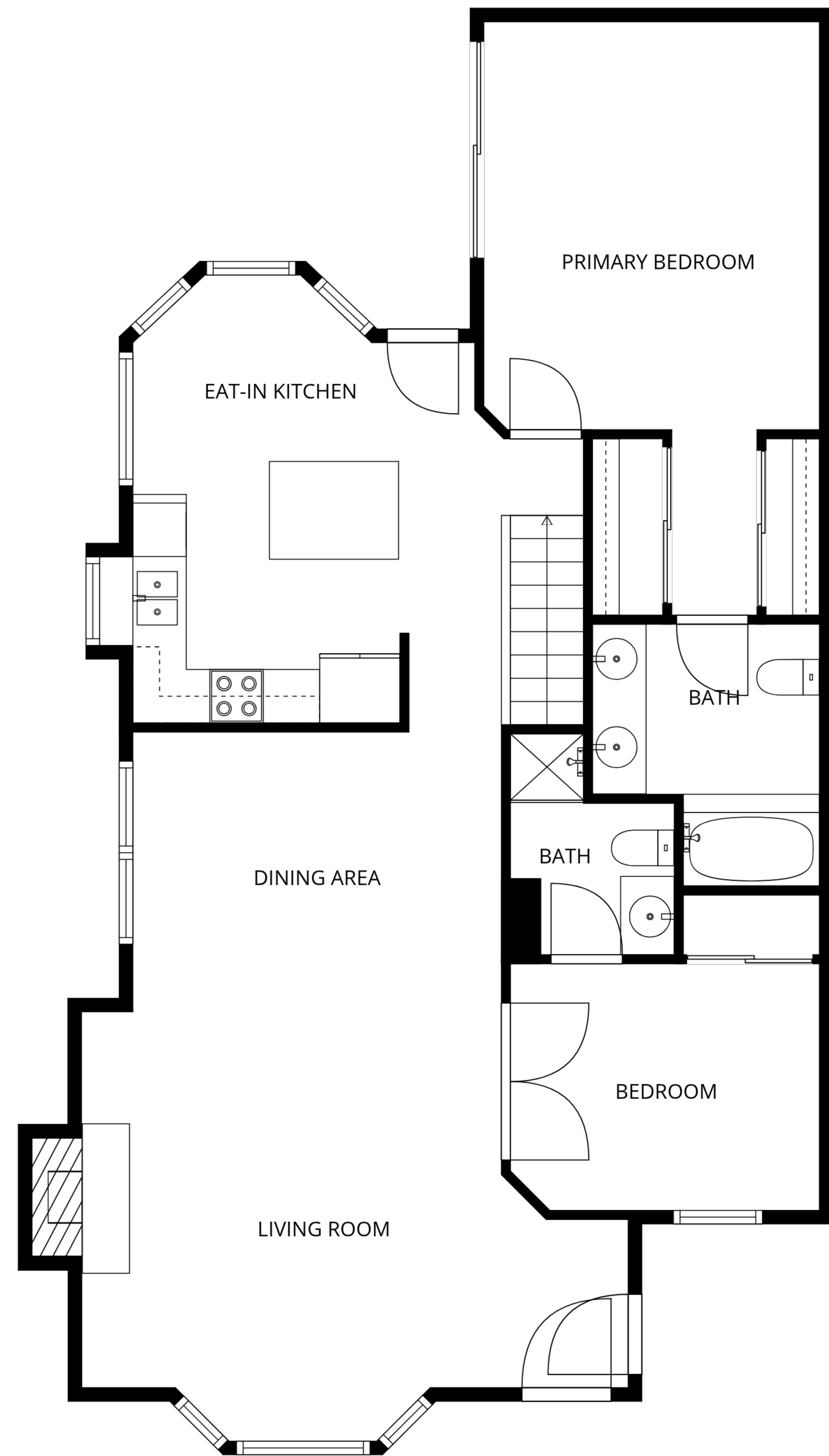
2nd floor
