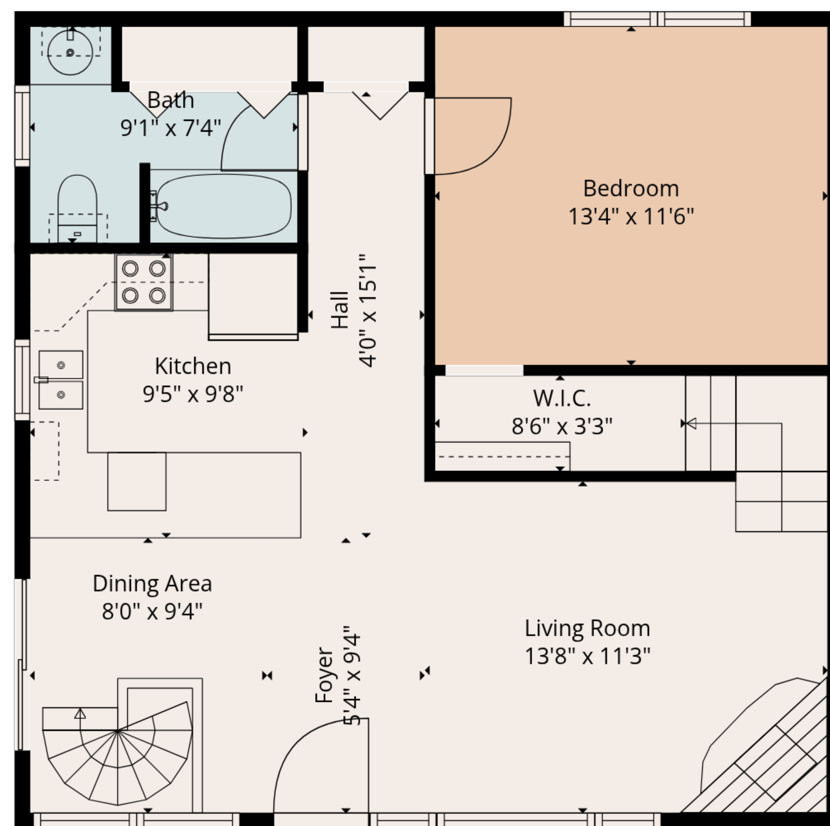
2nd Floor
