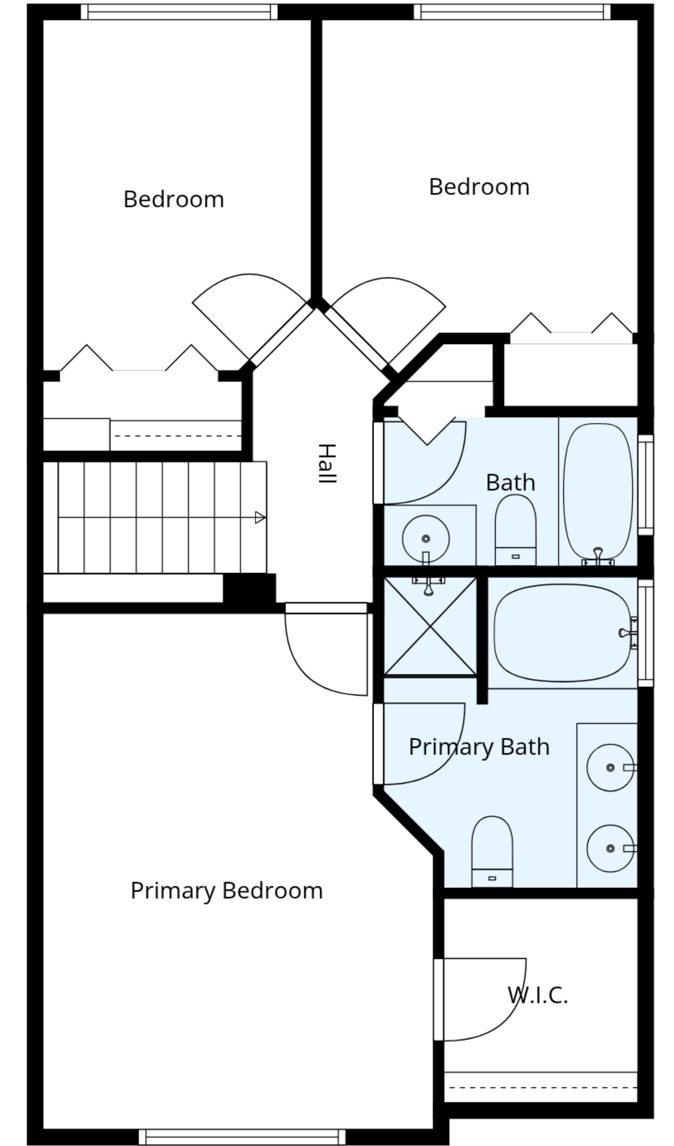
2nd Floor
