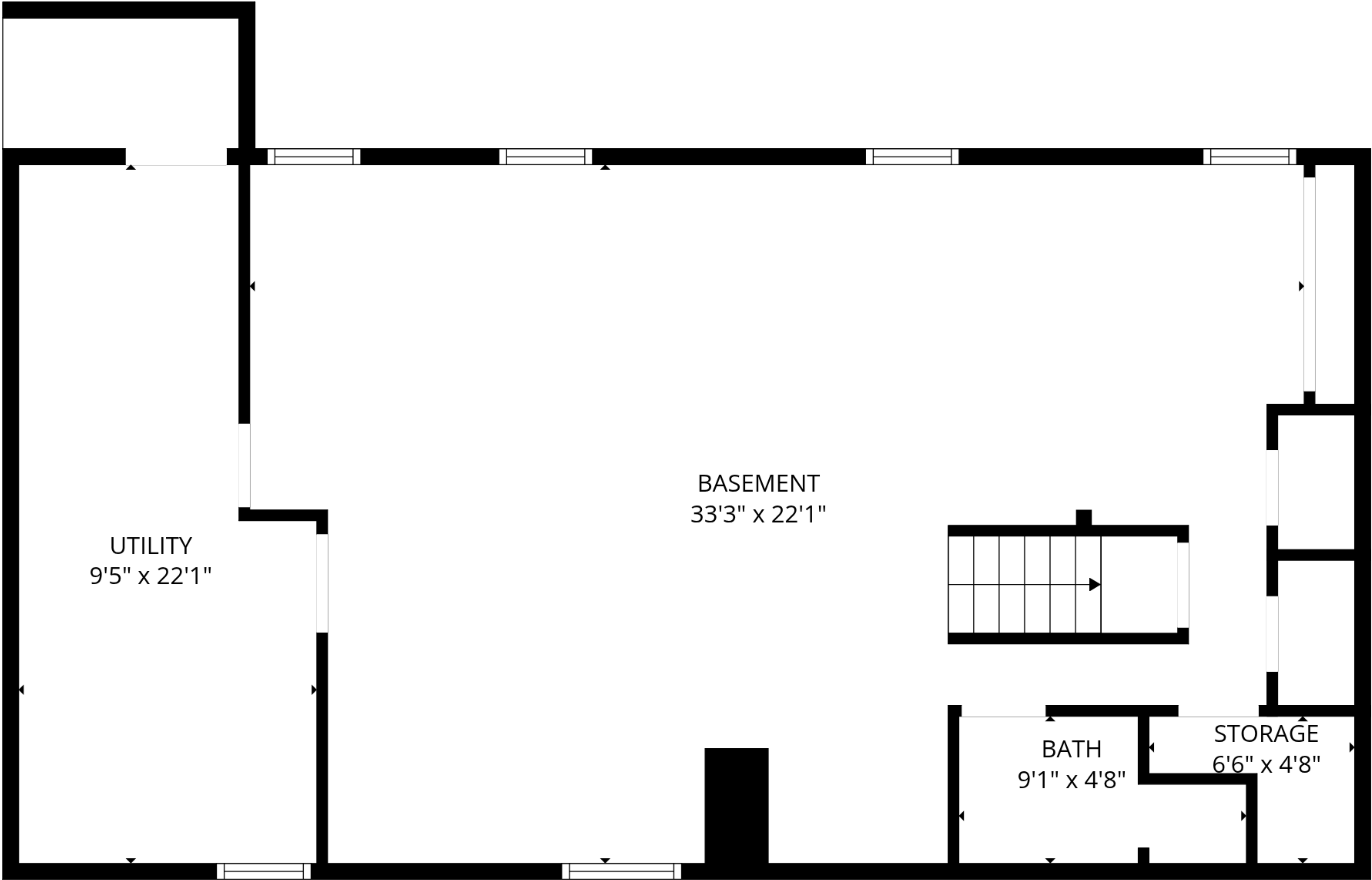
FLOOR 1
