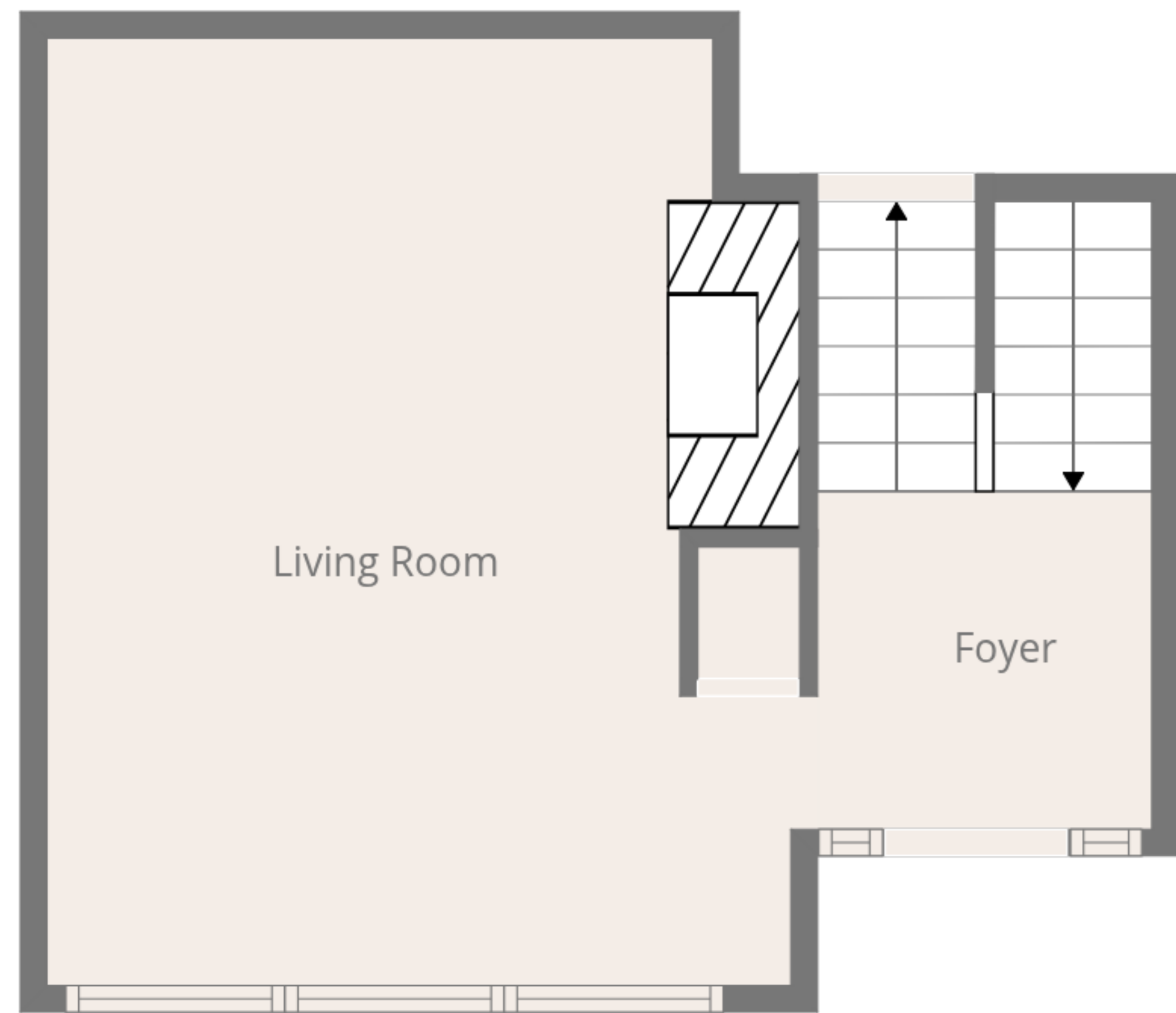
2nd Floor
