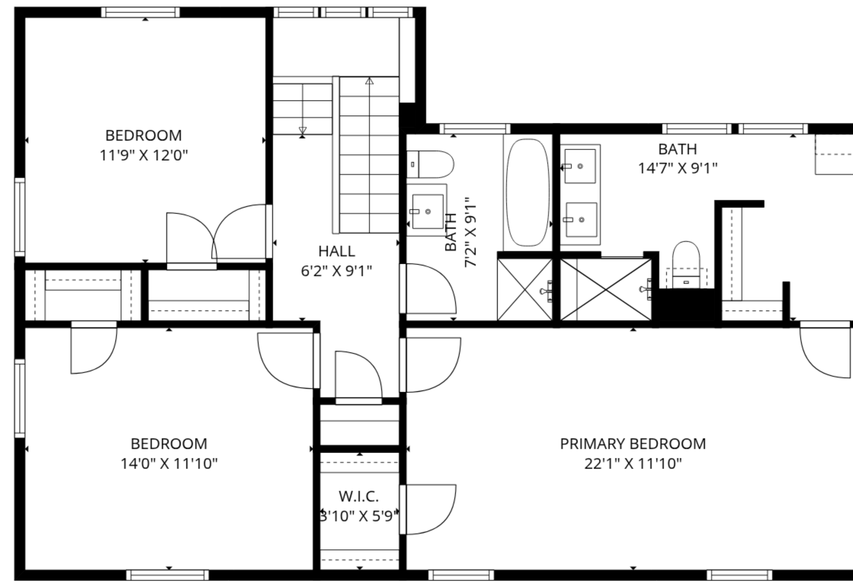
3RD FLOOR
