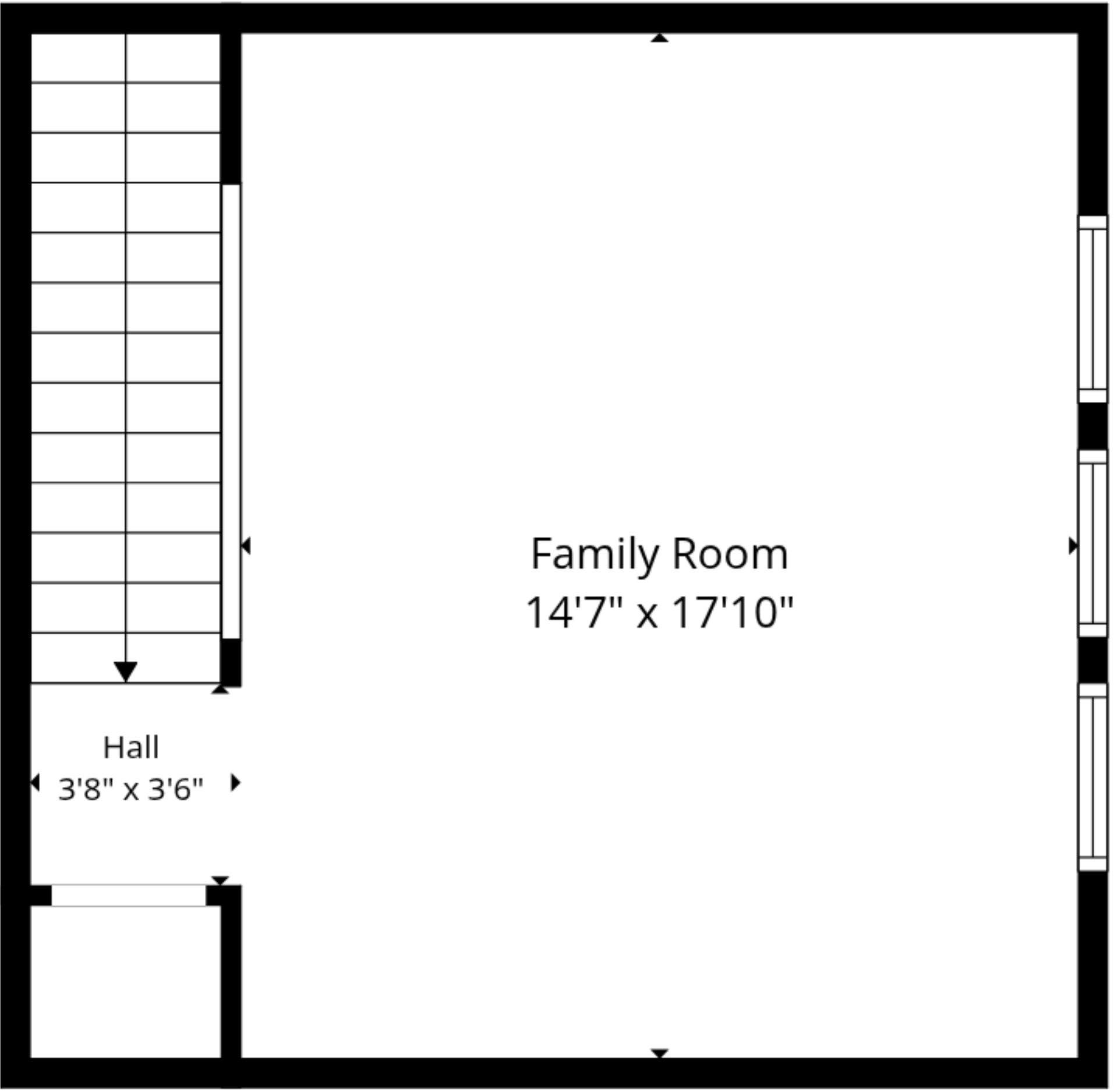
2nd Floor
