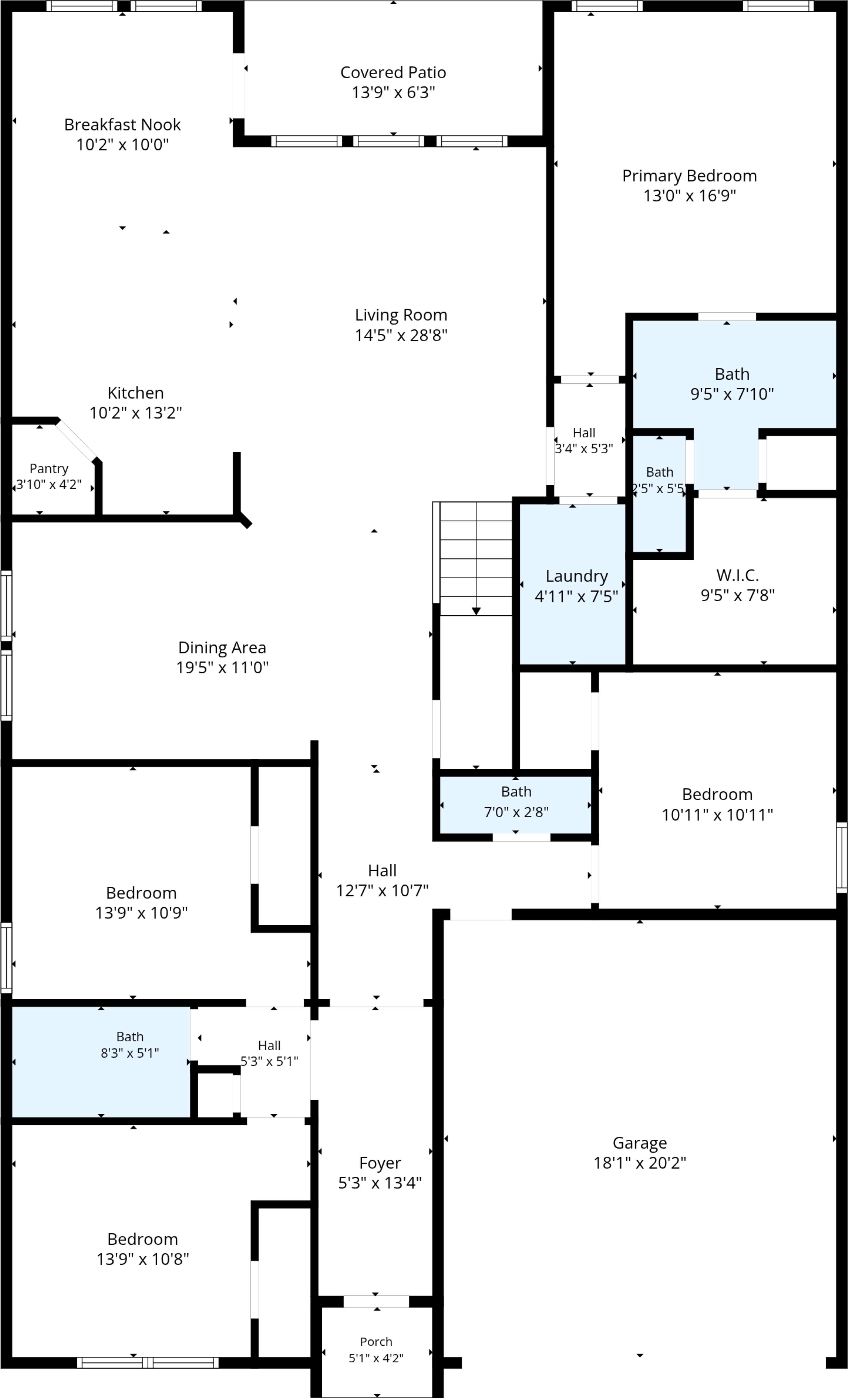
1st Floor
