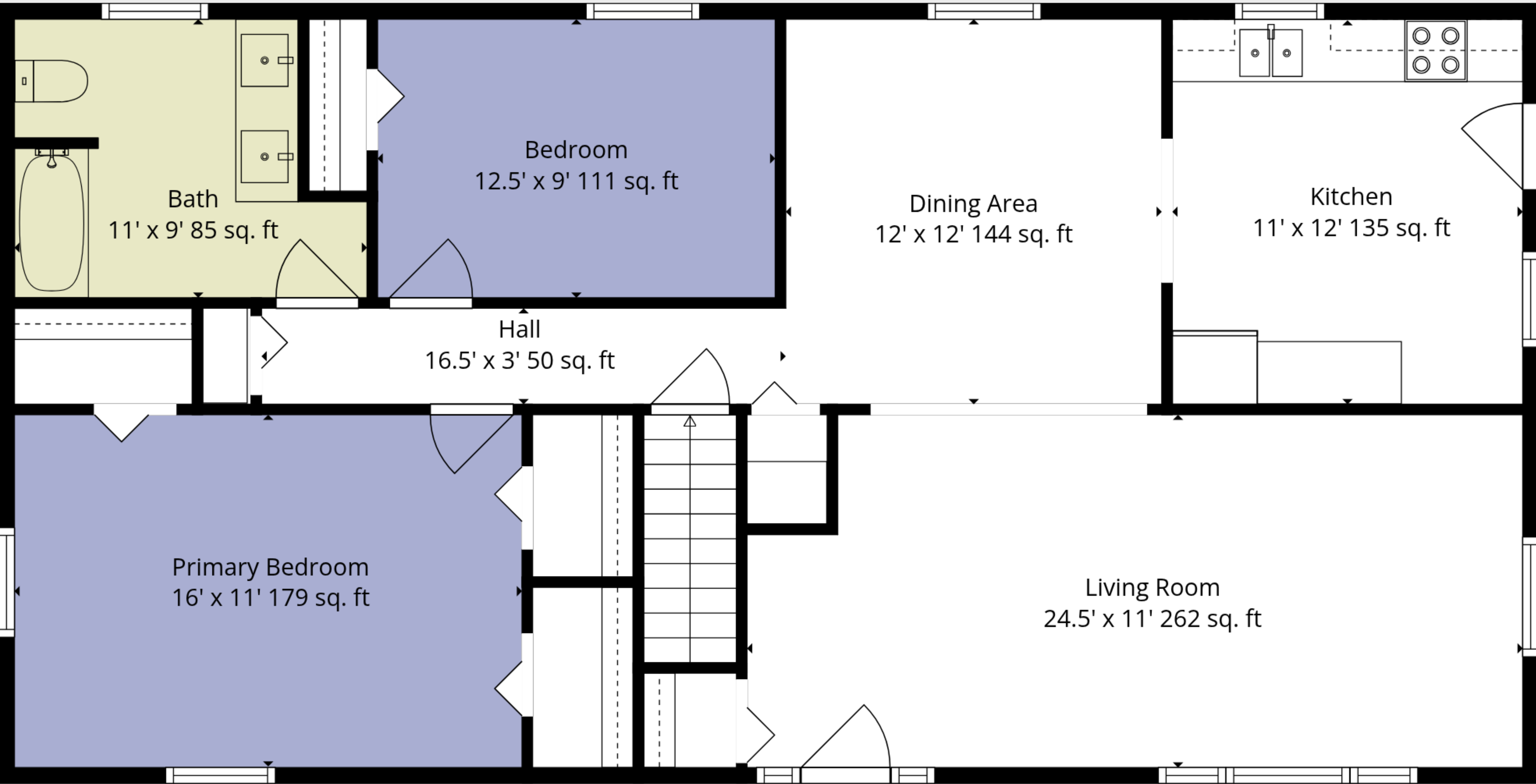
2nd Floor
