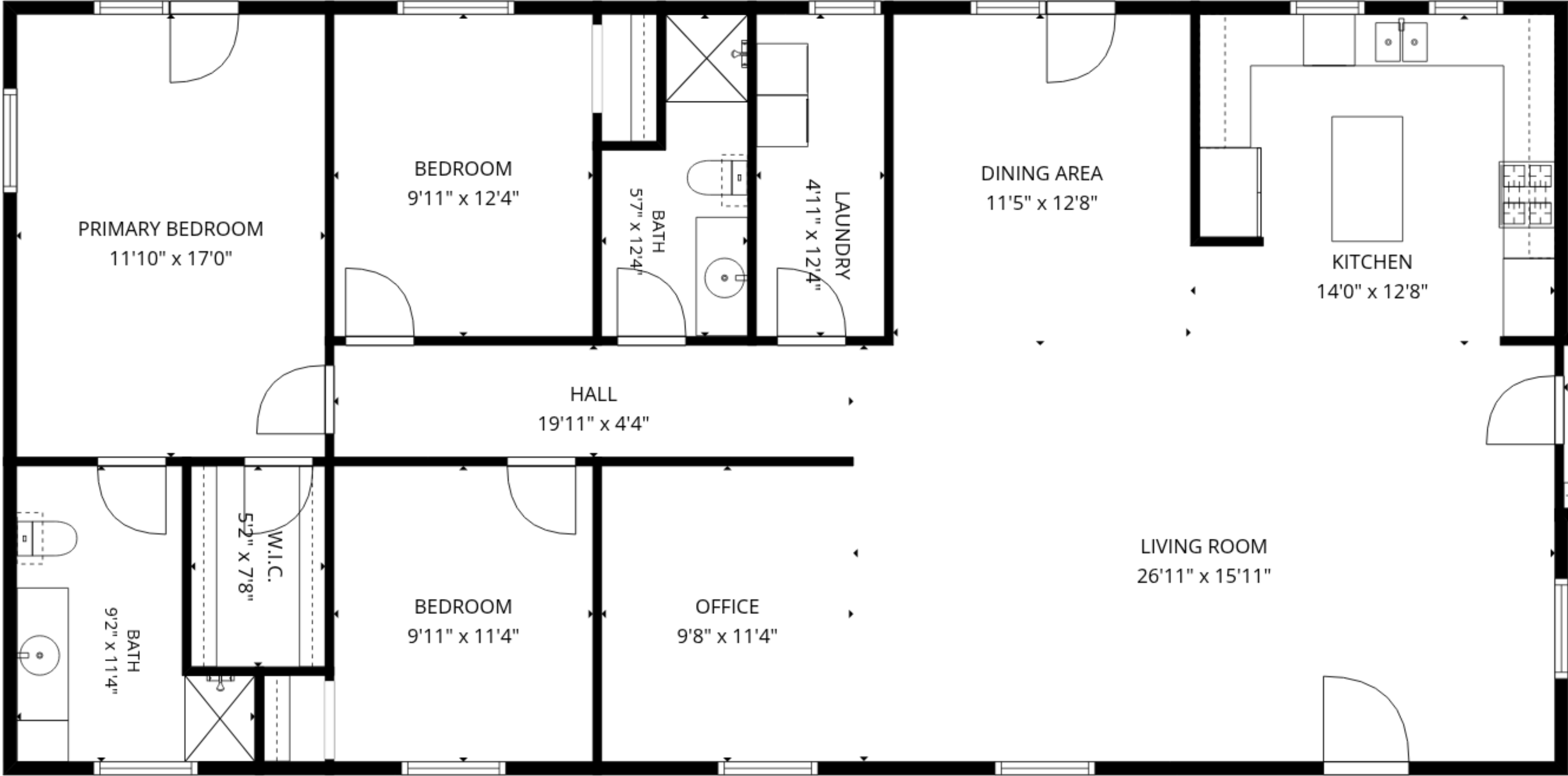
2nd floor
