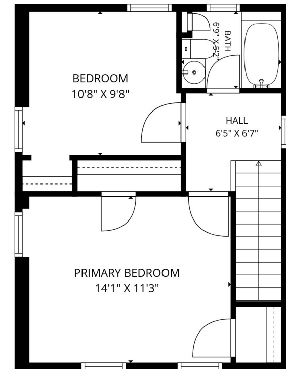
2ND FLOOR
