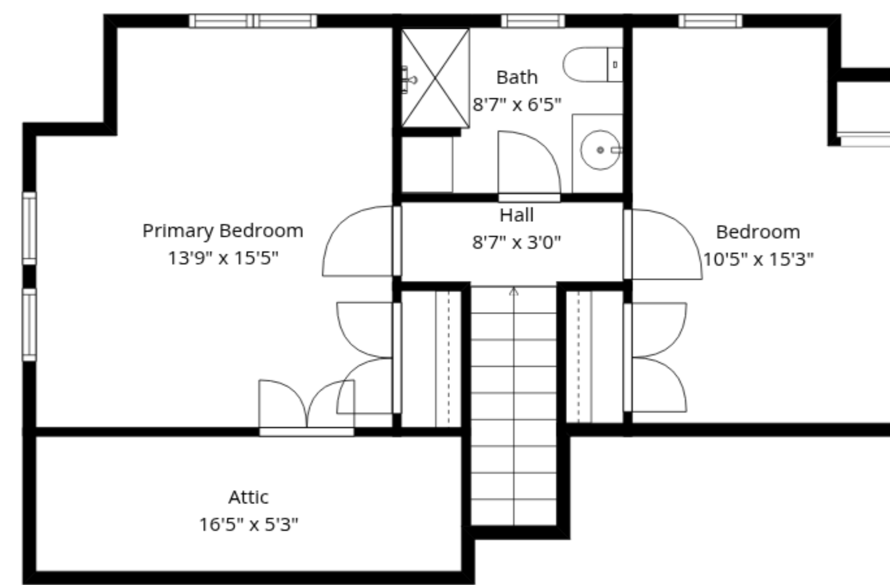
2nd Floor
