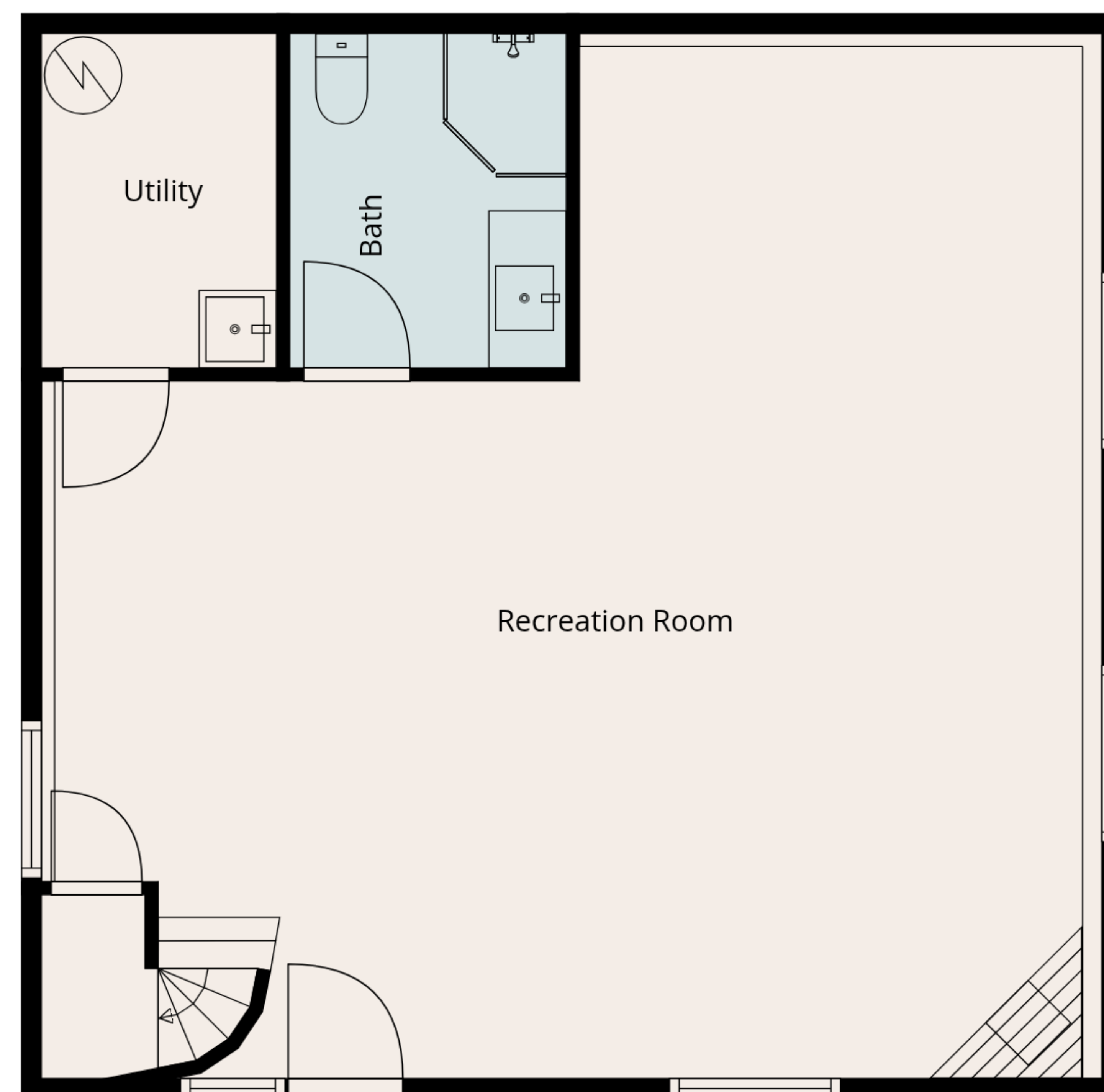
2nd Floor
