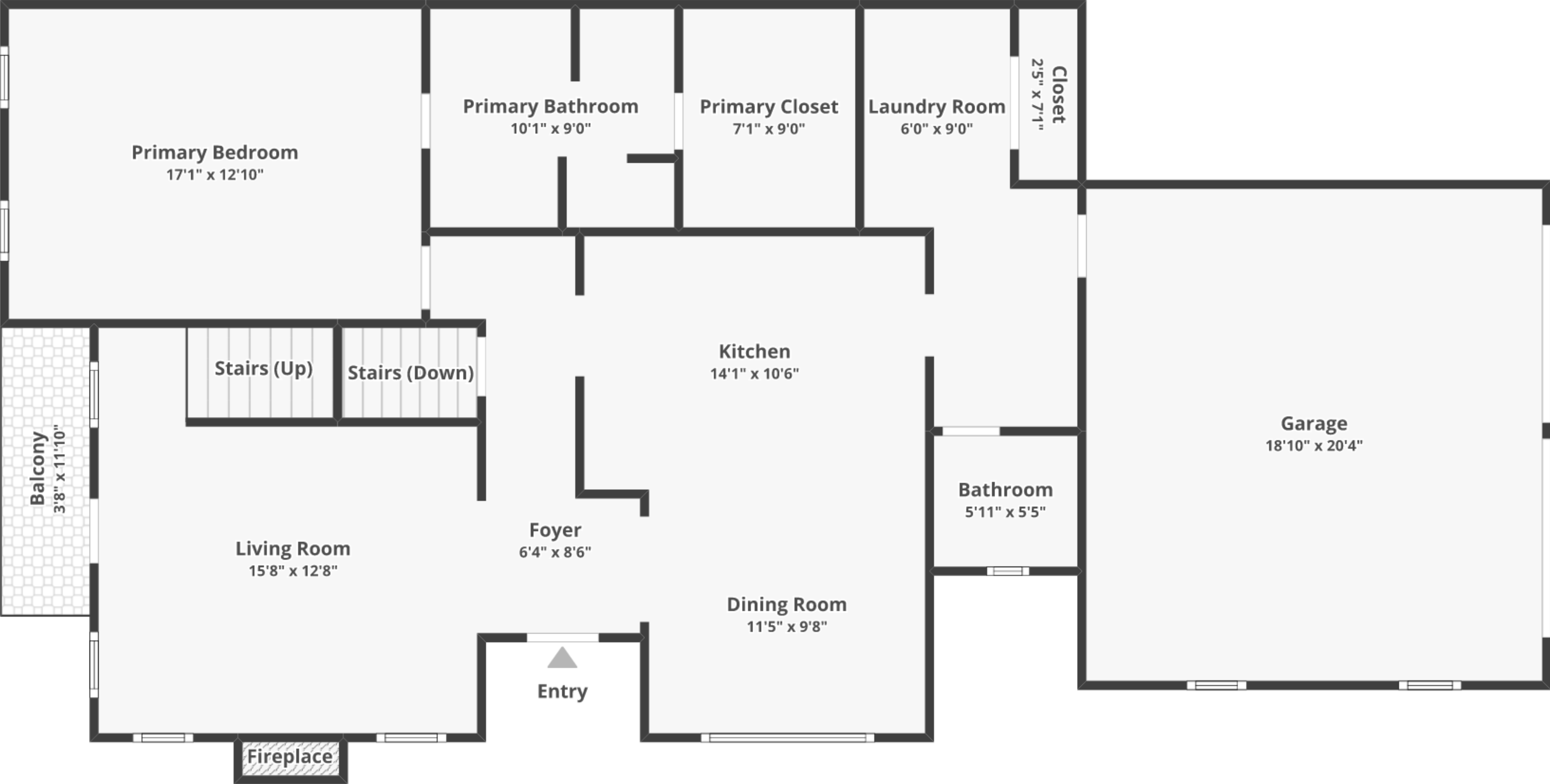
FLOOR 1
