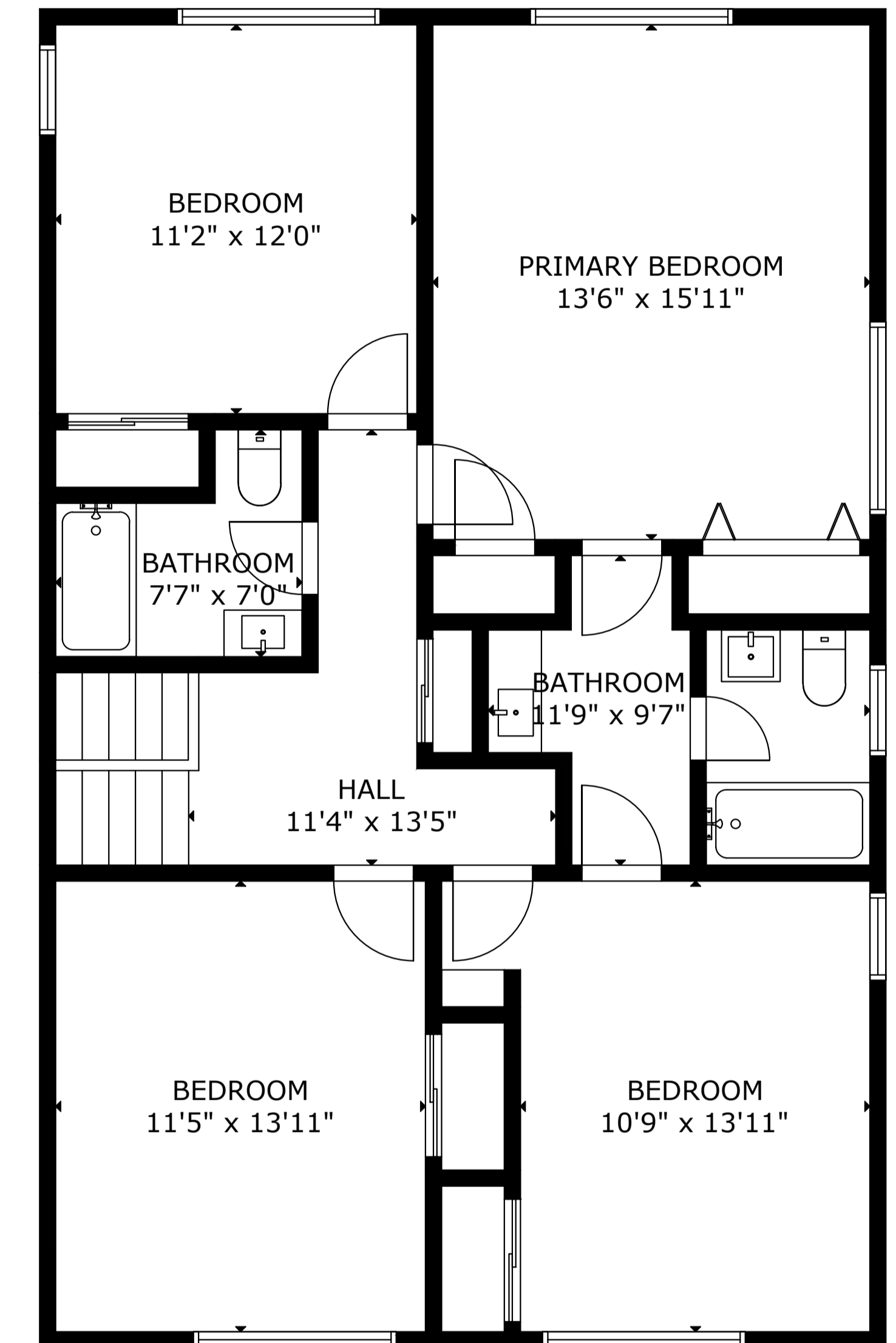
UPPER LEVEL 1
