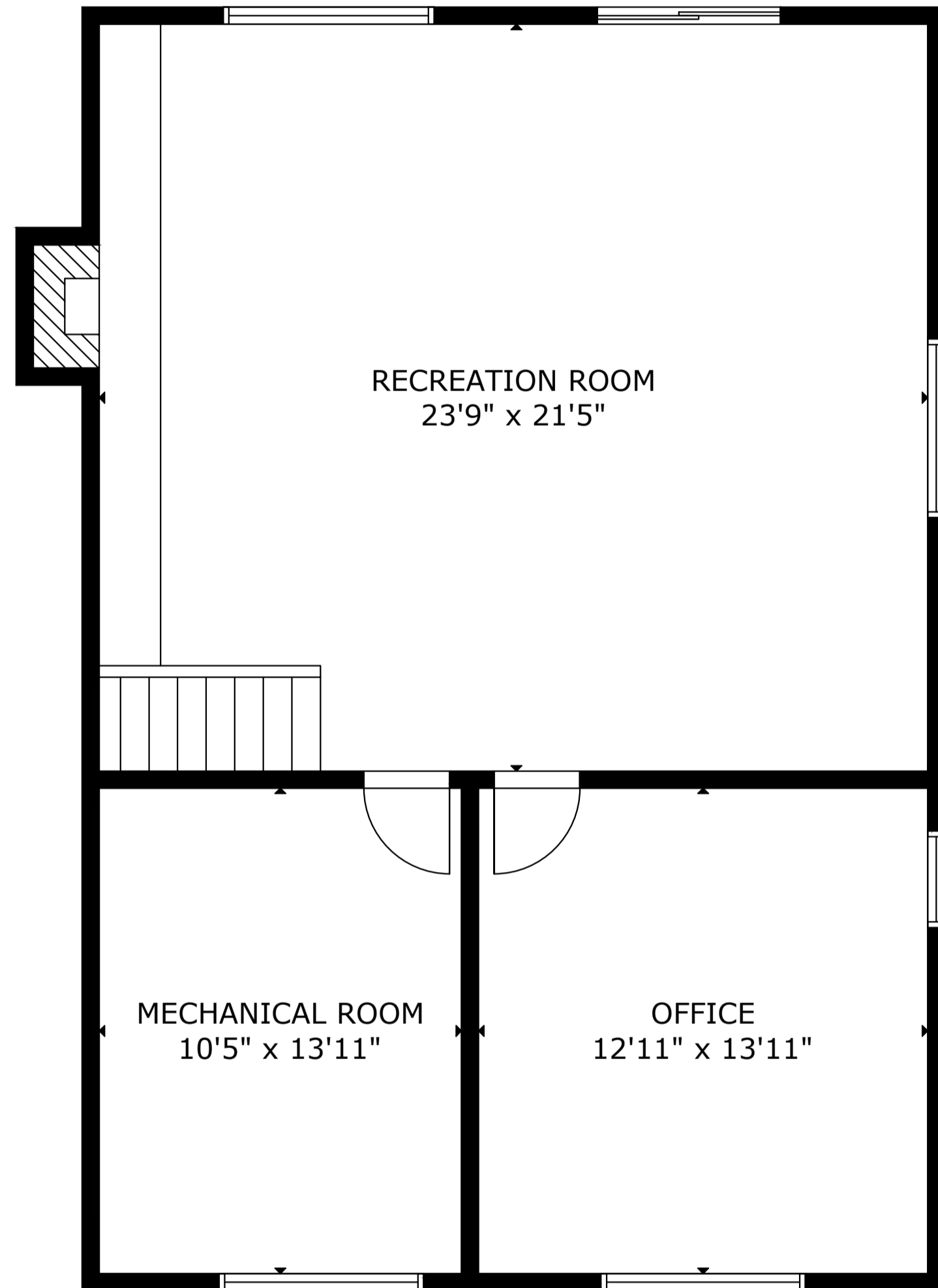
LOWER FLOOR
