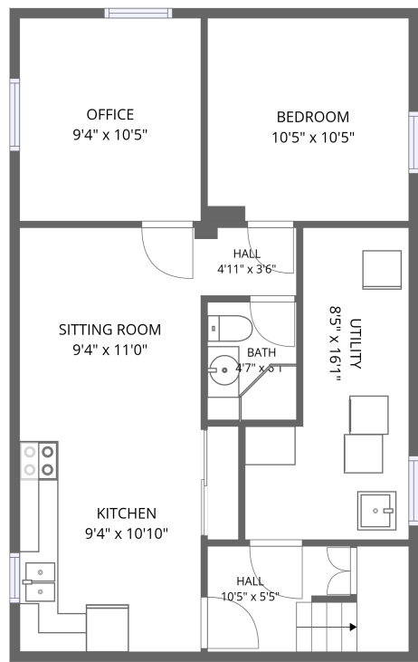
Basement
