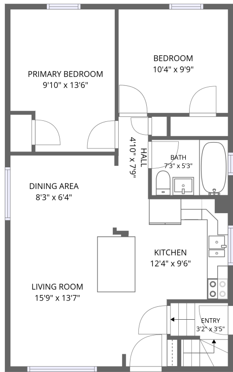
1st floor
