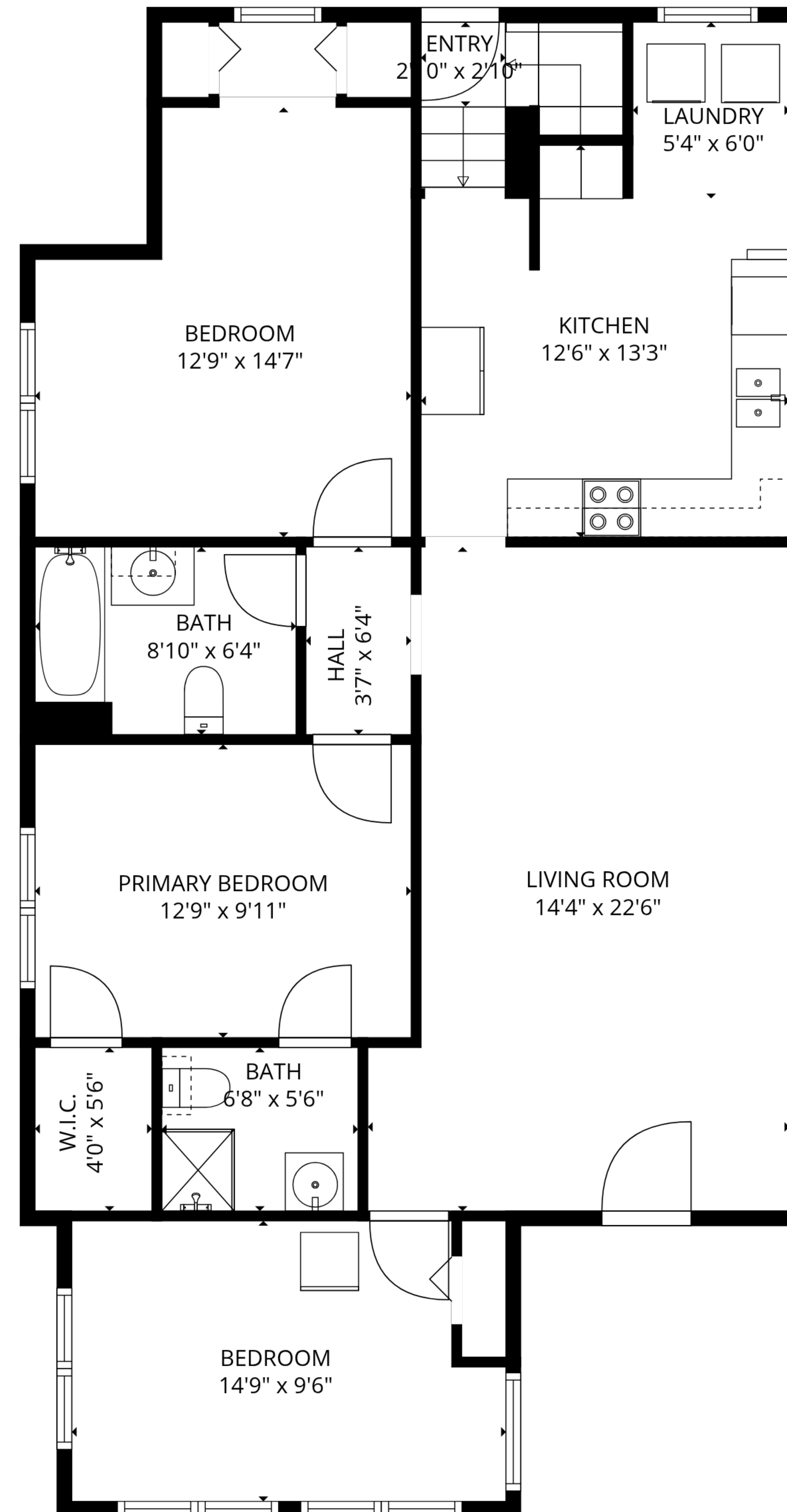
1st floor
