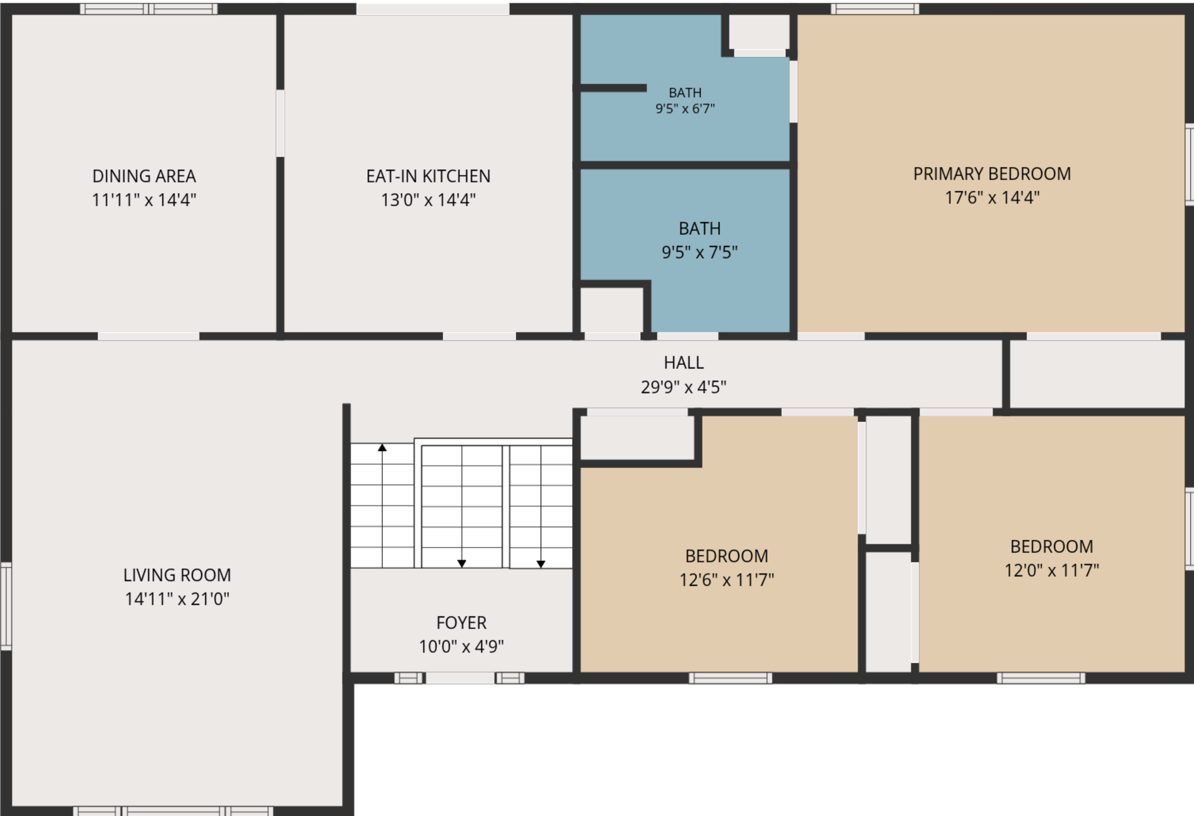
2ND FLOOR
