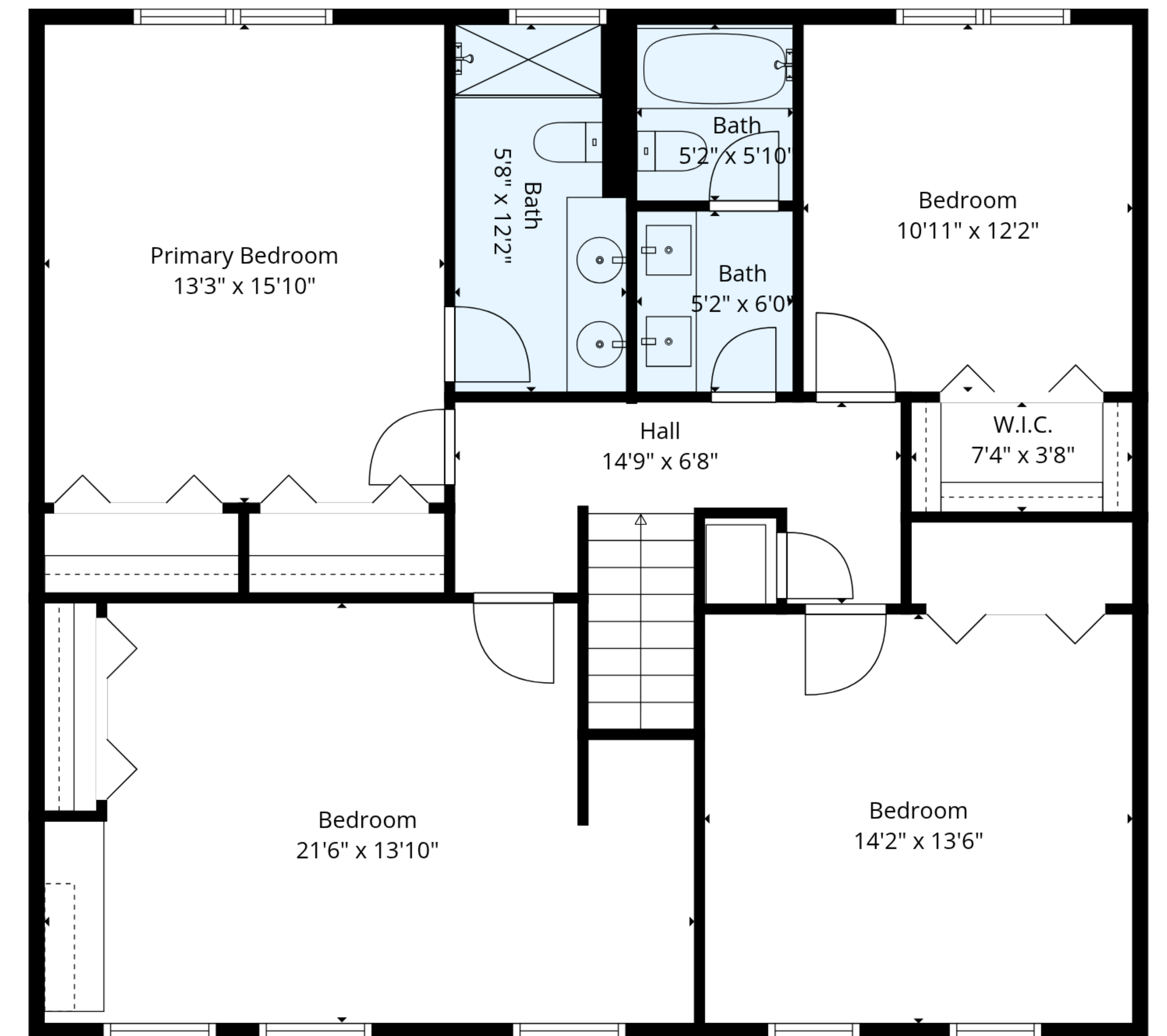
2nd Floor
