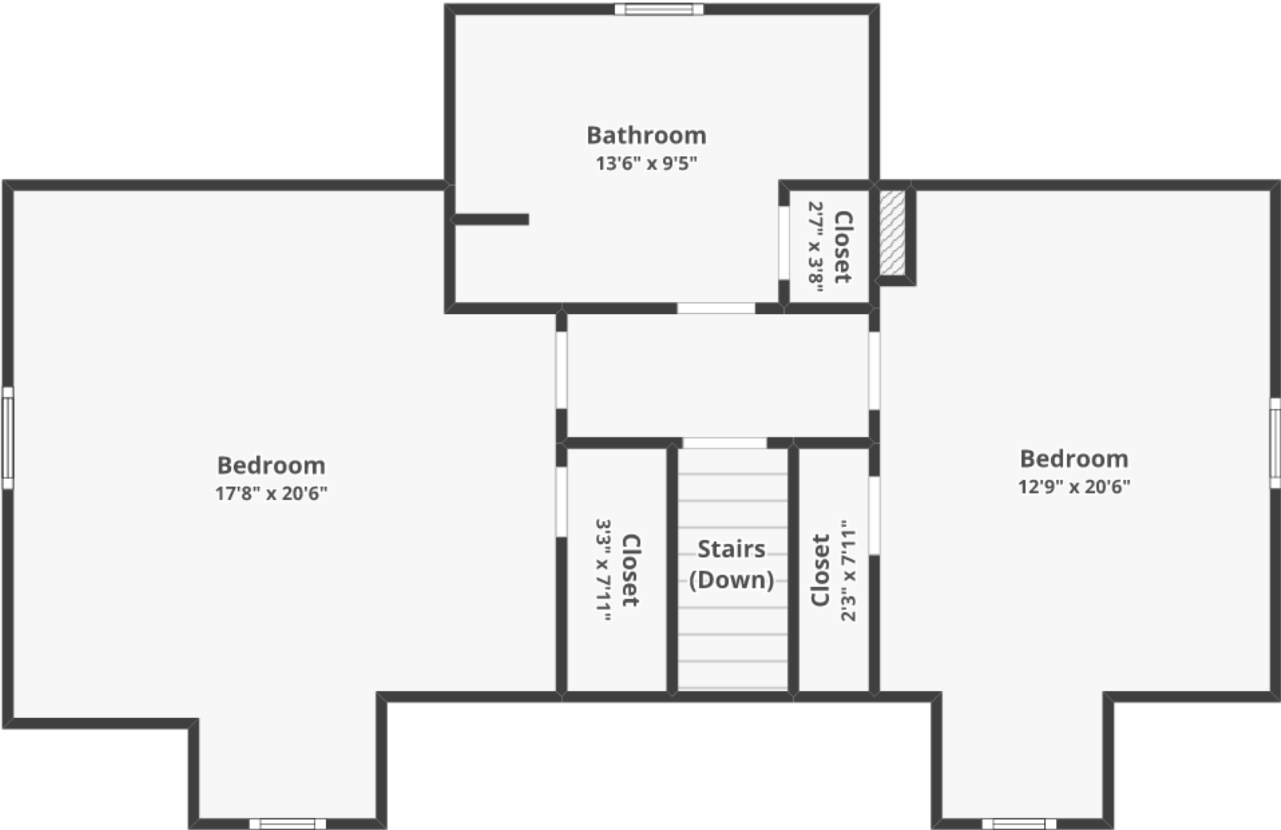
FLOOR 2
