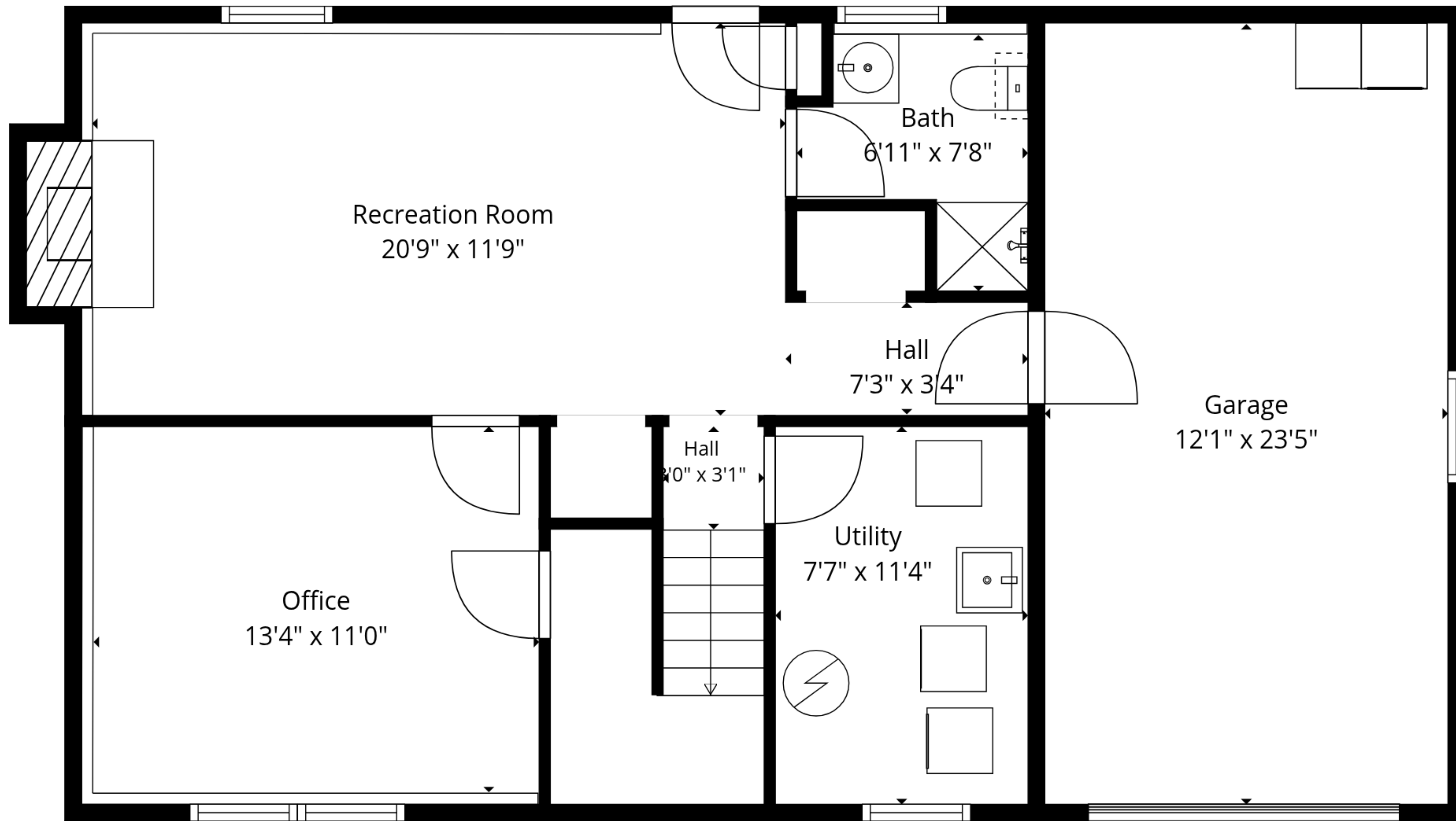
1st Floor
