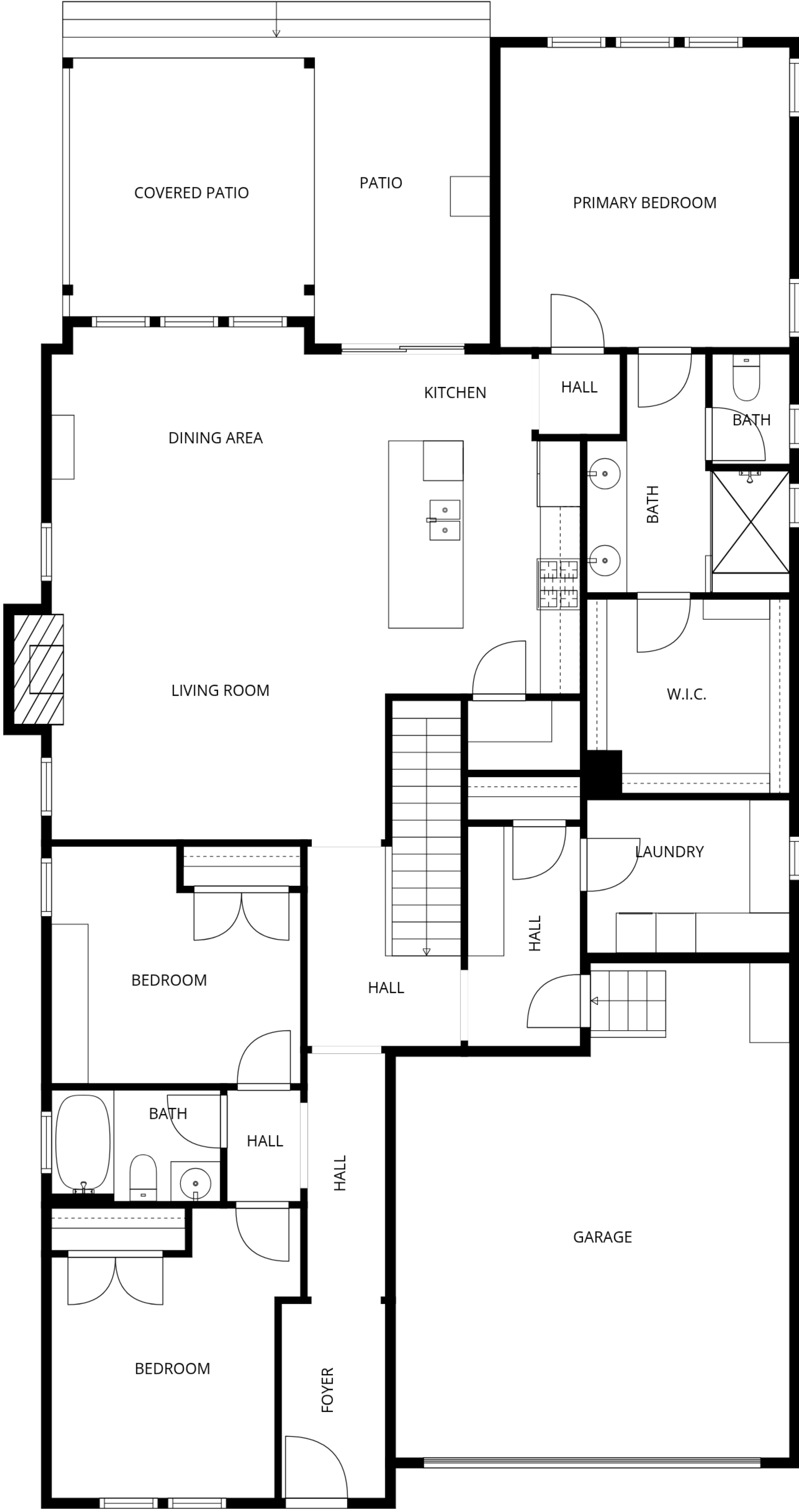
1st floor
