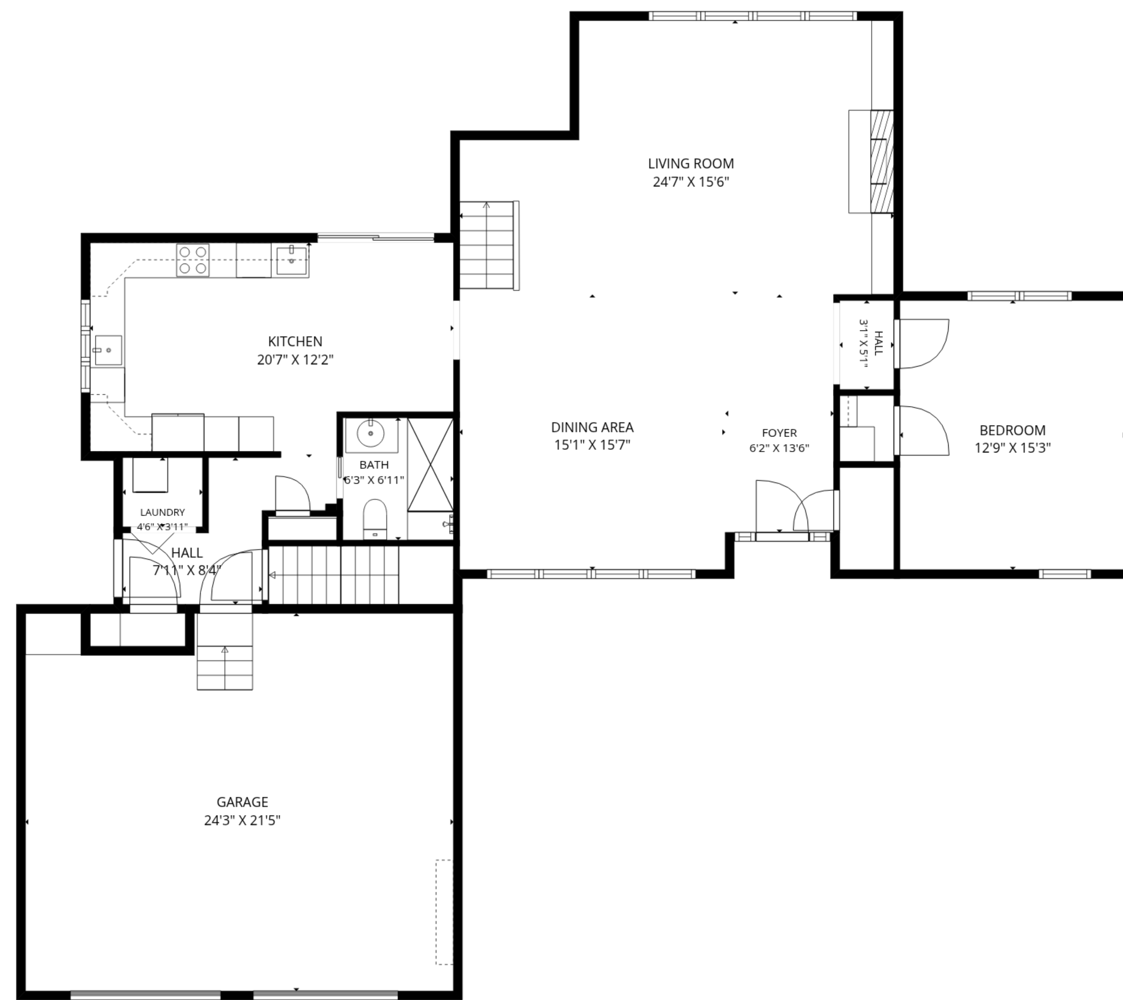
1ST FLOOR
