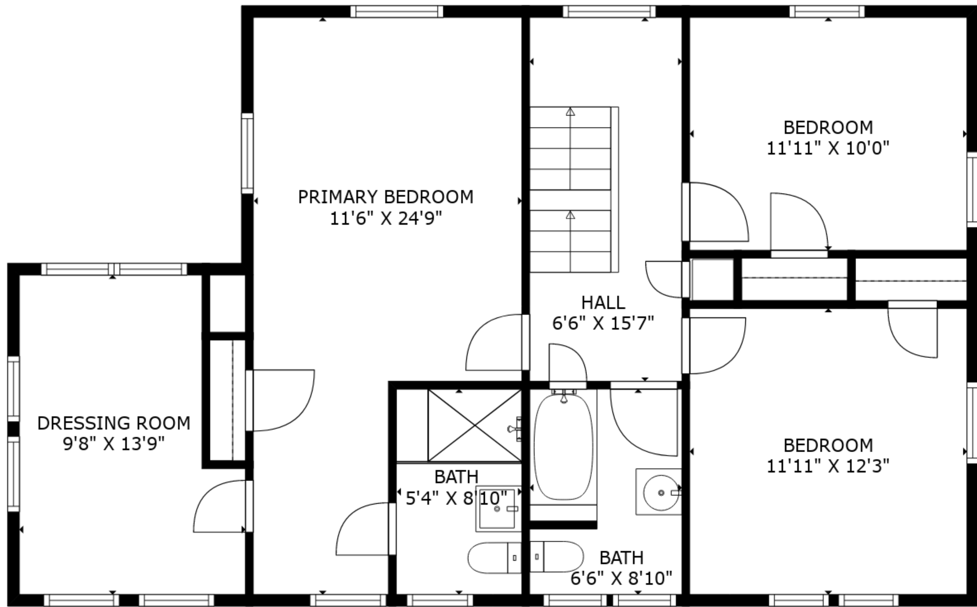
SECOND FLOOR
