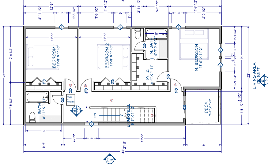
PROPOSED 2ND FLOOR PLAN SCALE: 1/4"=1'
