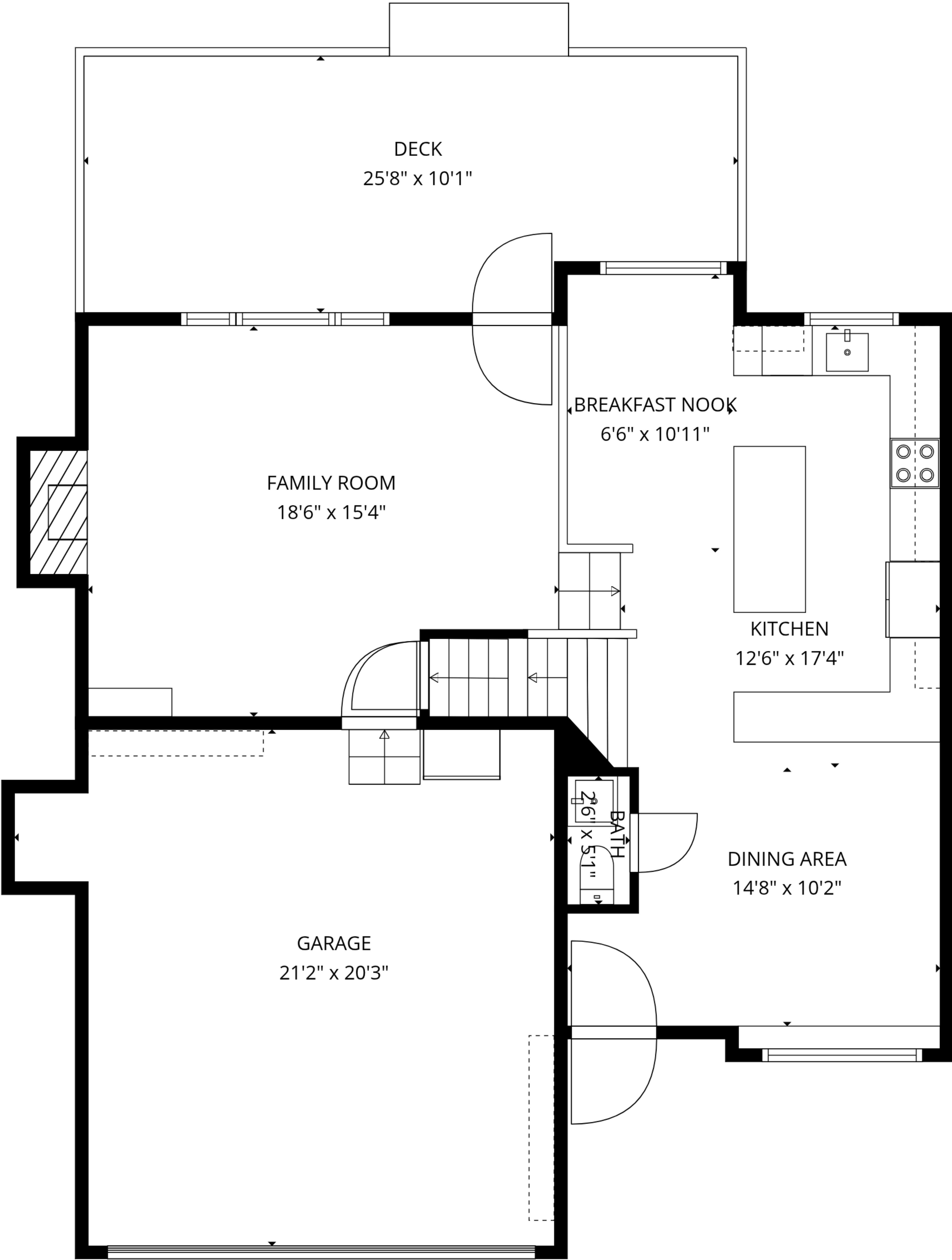
FLOOR 2
