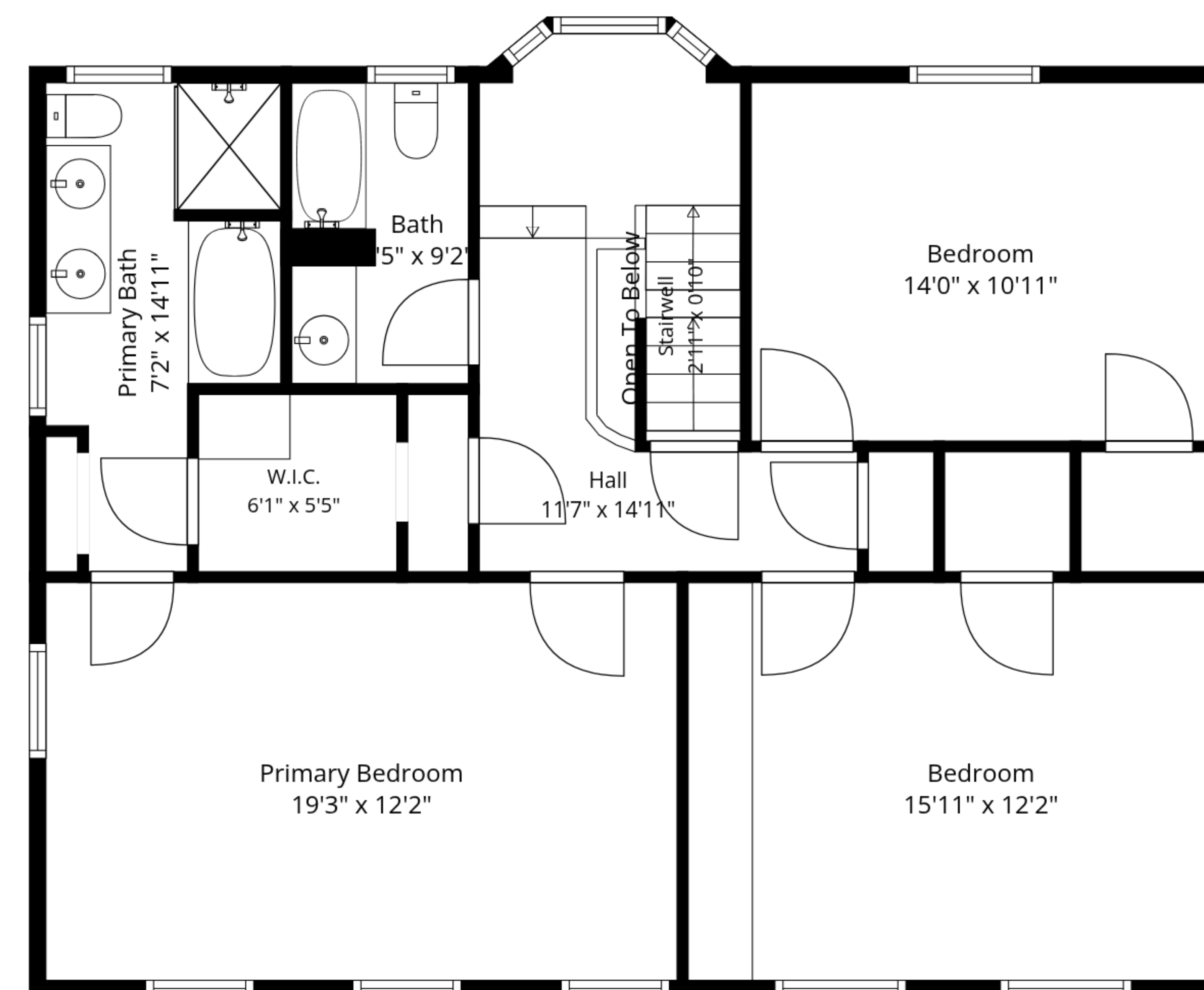
2nd Floor
