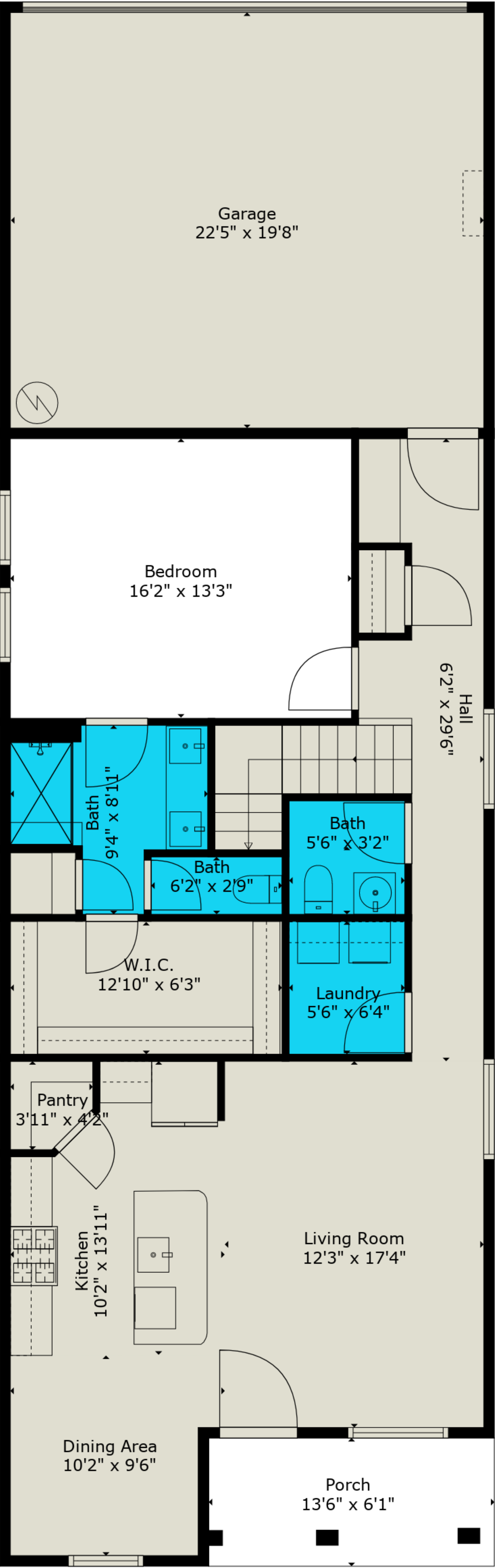
Floor 1
