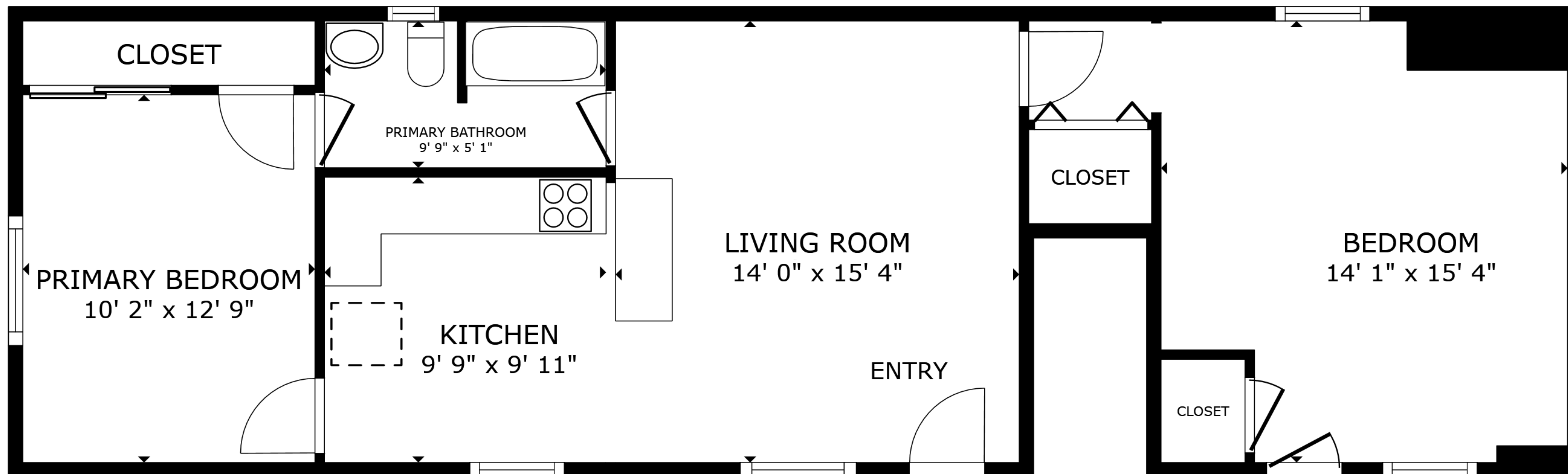
FLOOR PLAN
