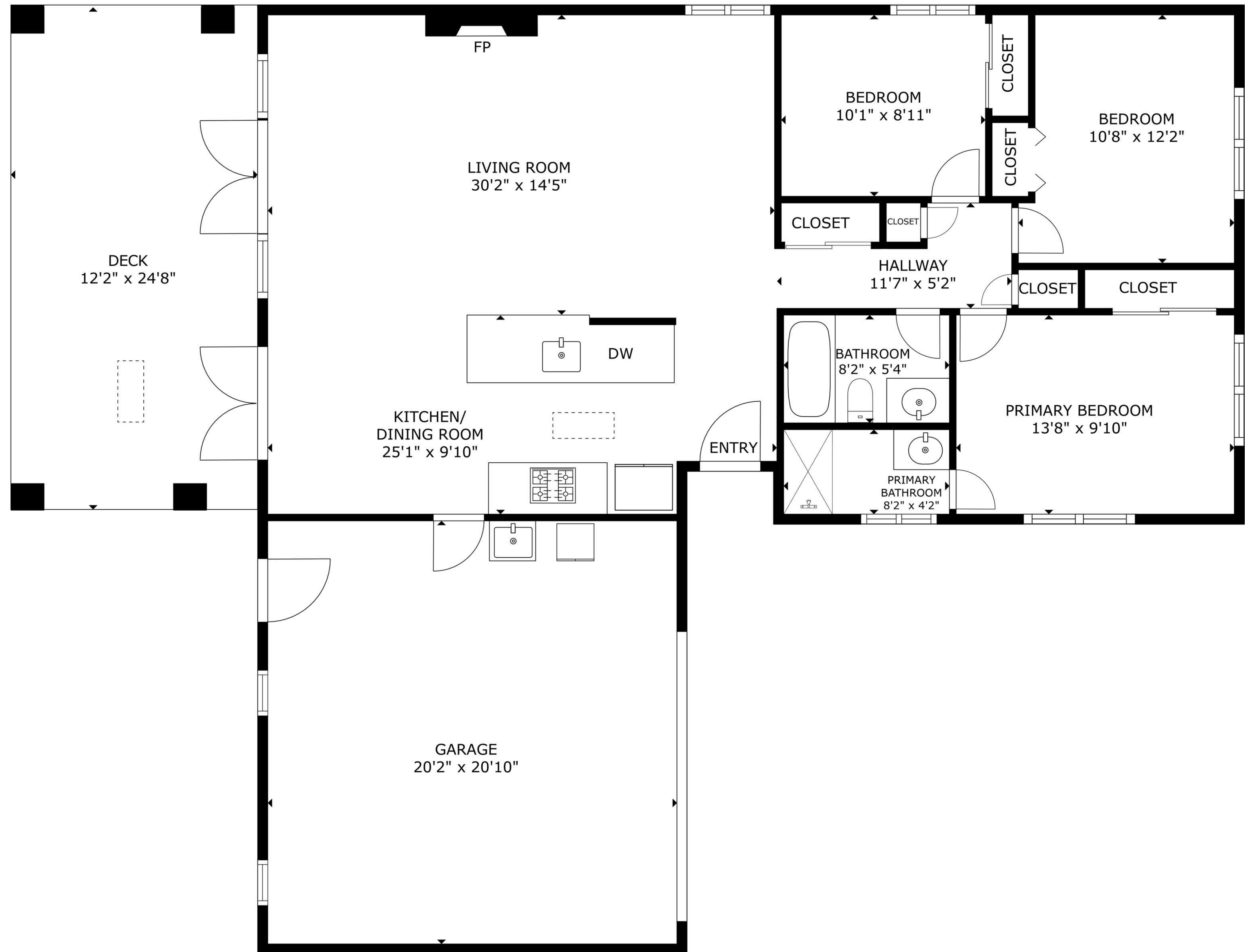
FLOOR PLAN
