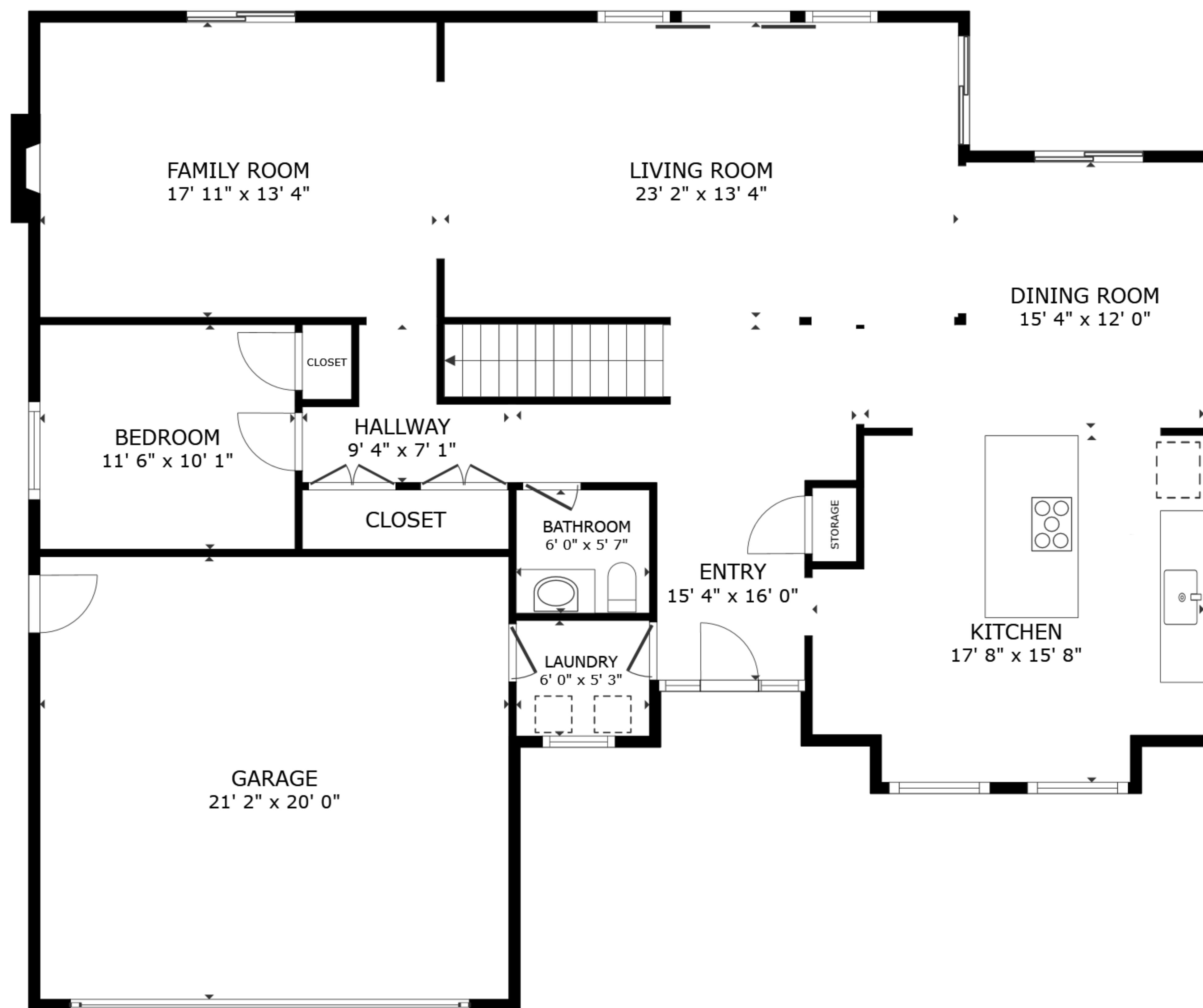
FLOOR 1
