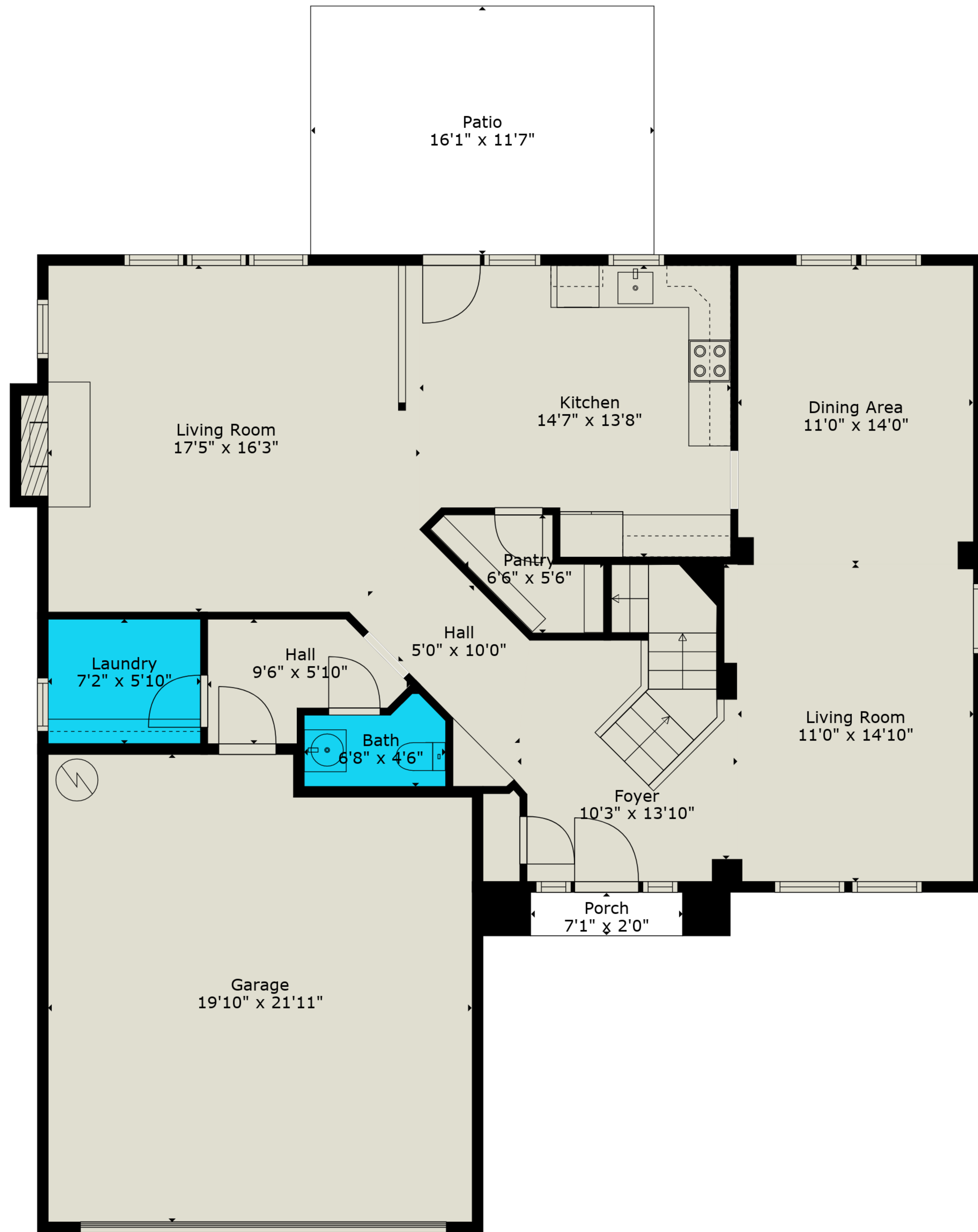
Floor 1
