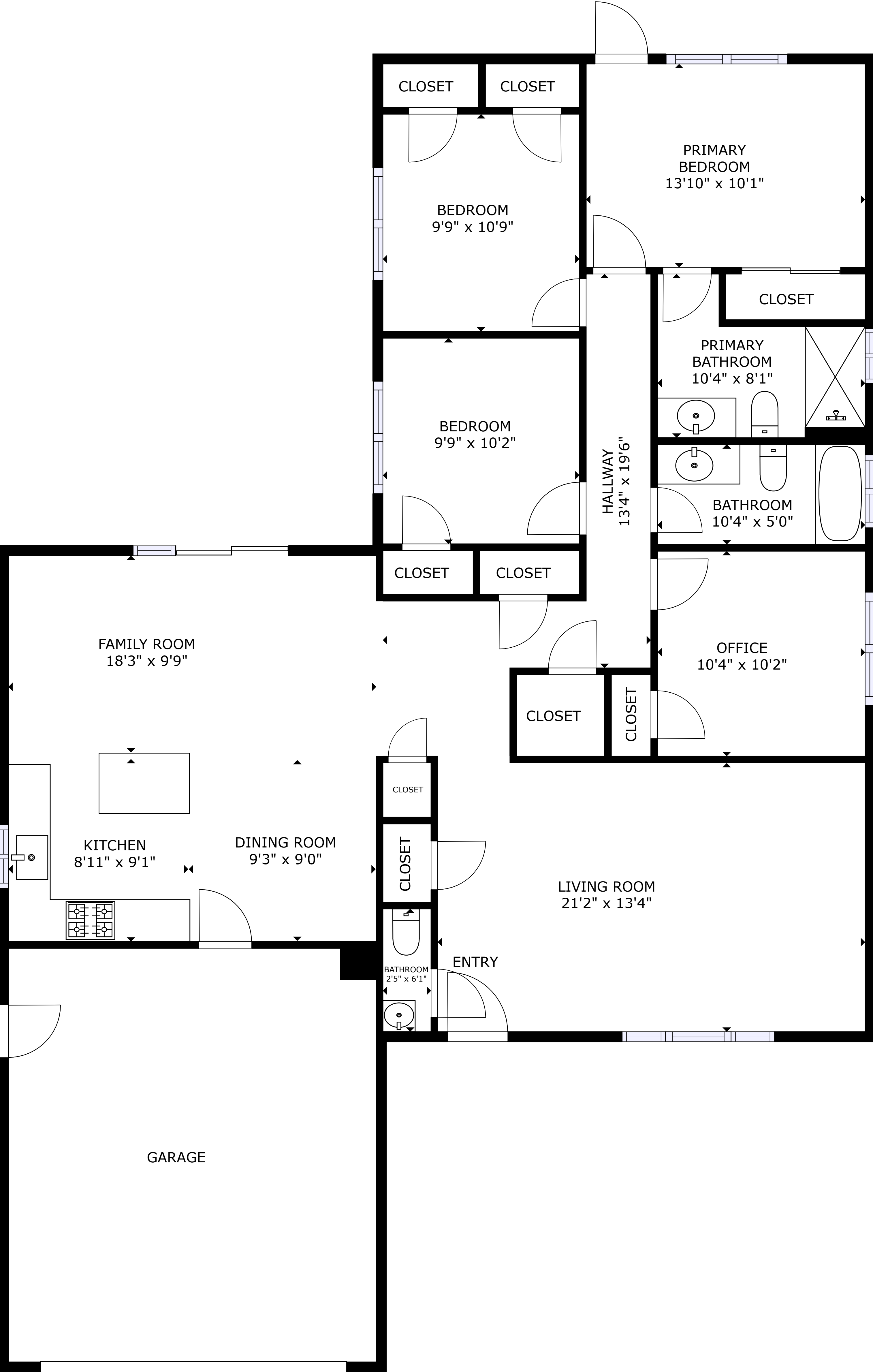
FLOOR PLAN
