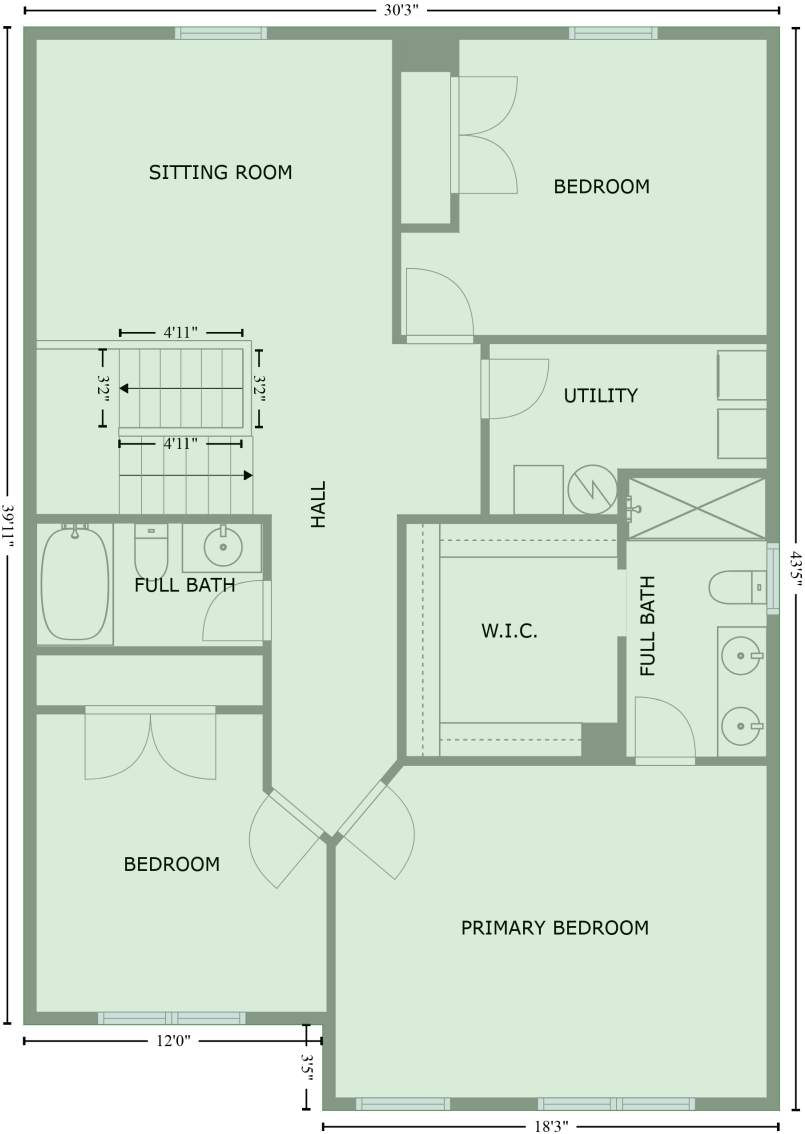
FLOOR 2 [AREA: 1272]
