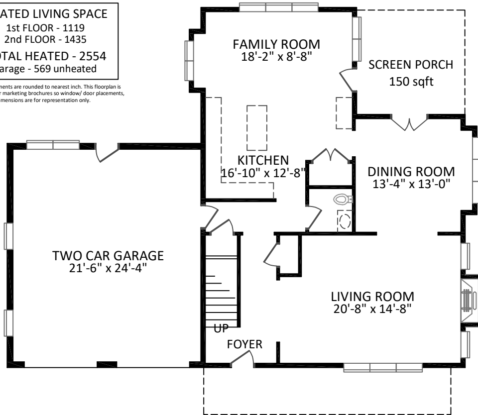
1ST FLOOR
