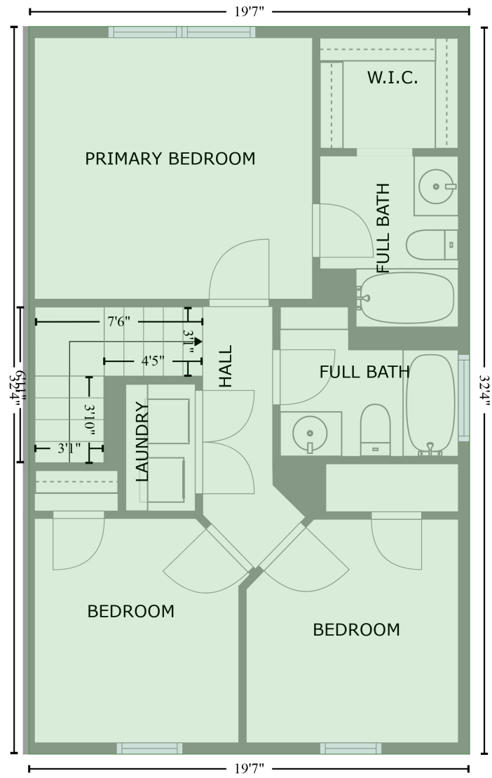
FLOOR 3 [AREA: 634]
