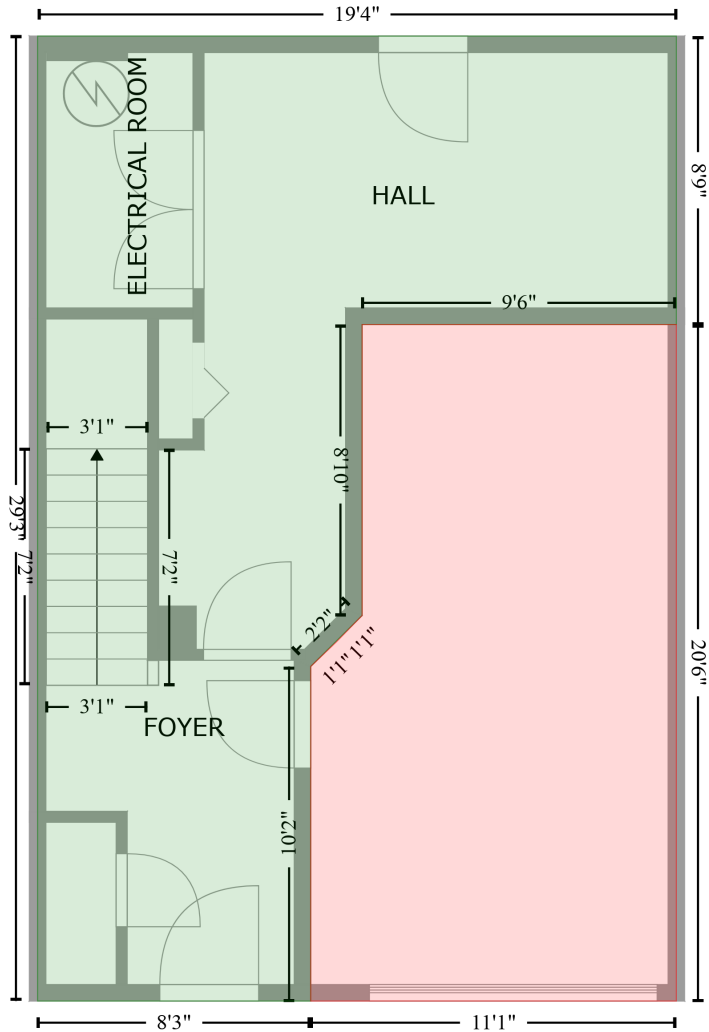
GARAGE (1) [AREA: 212]
