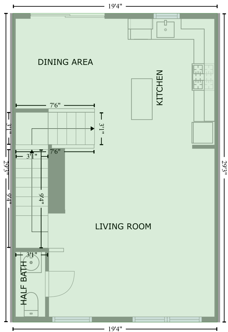
FLOOR 2 [AREA: 566]
