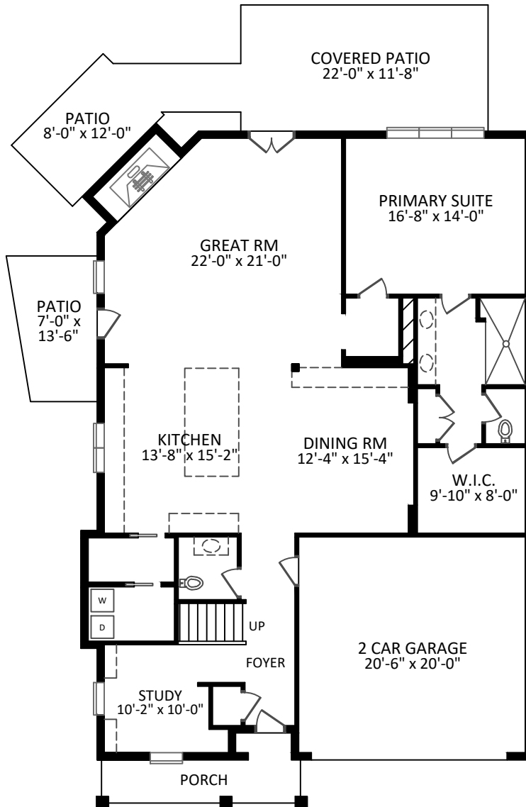
1ST FLOOR
