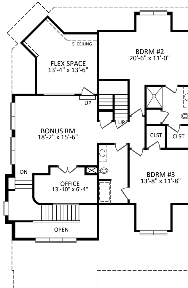
2ND FLOOR
