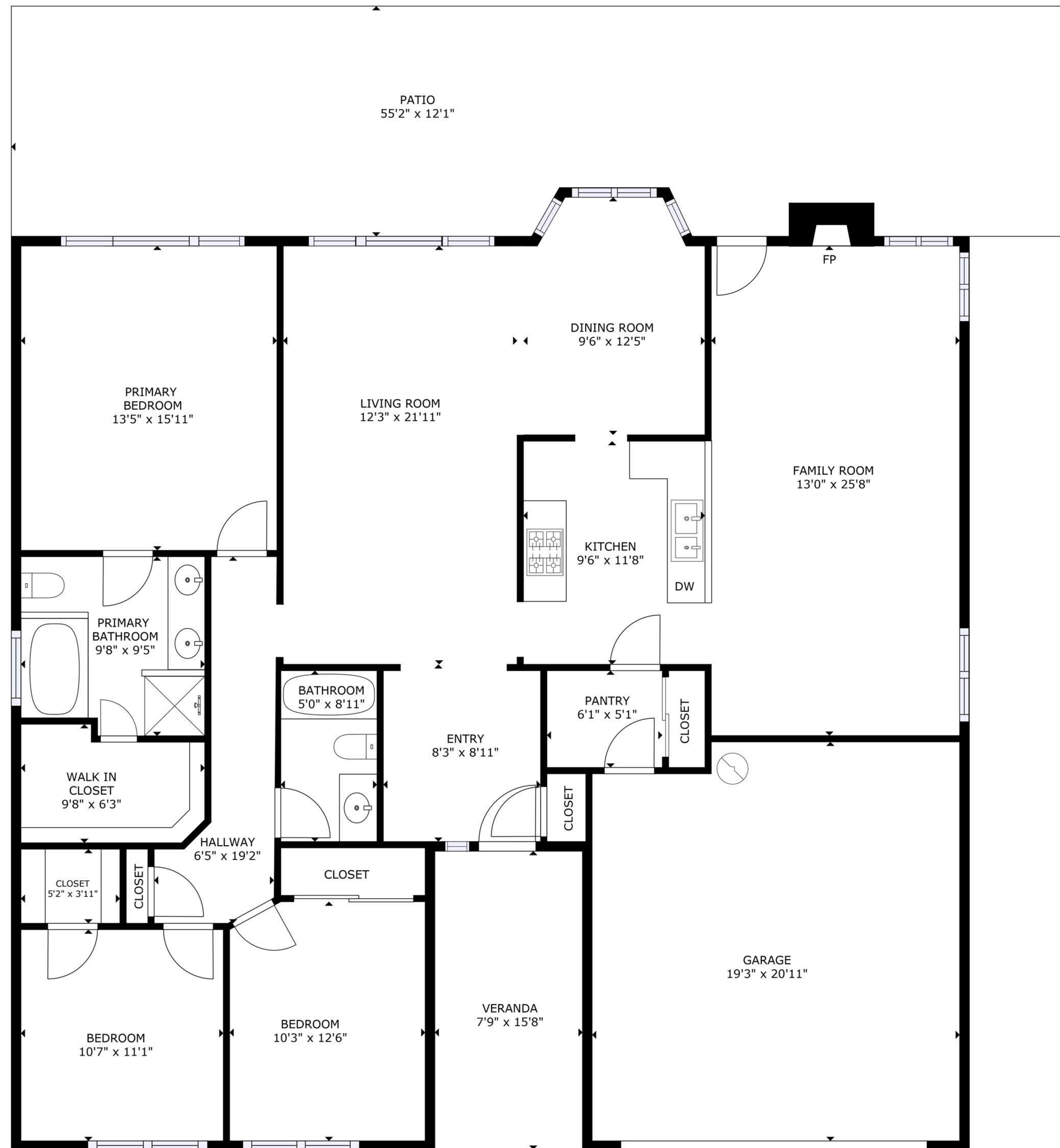
FLOOR PLAN
