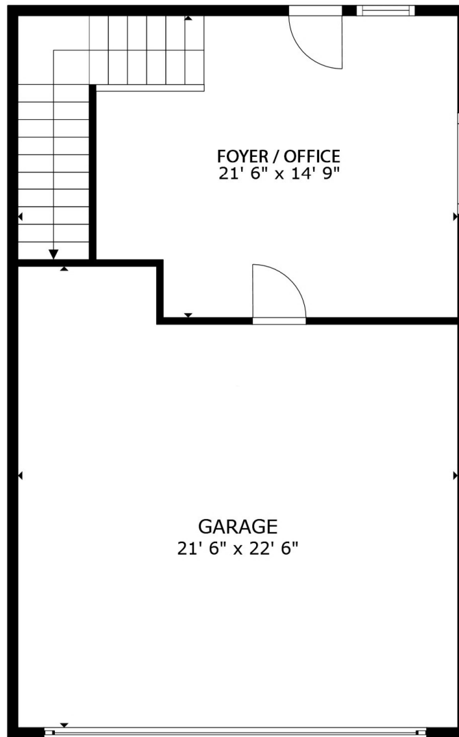
FLOOR 1
